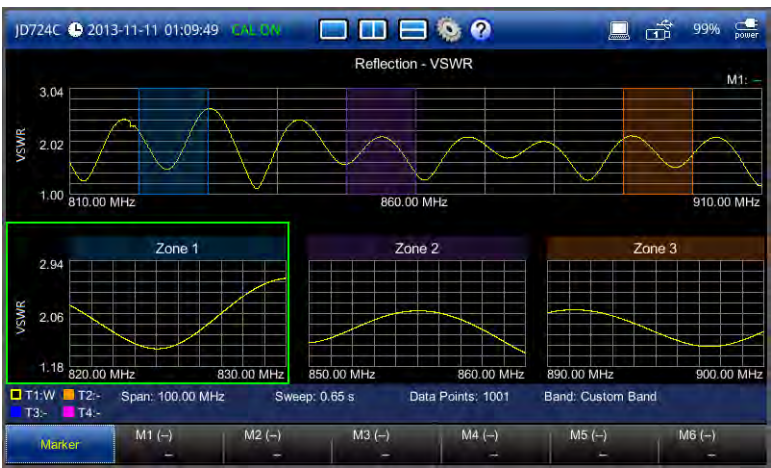
Figure 20 Reflection return loss measurement screen (single layout)
