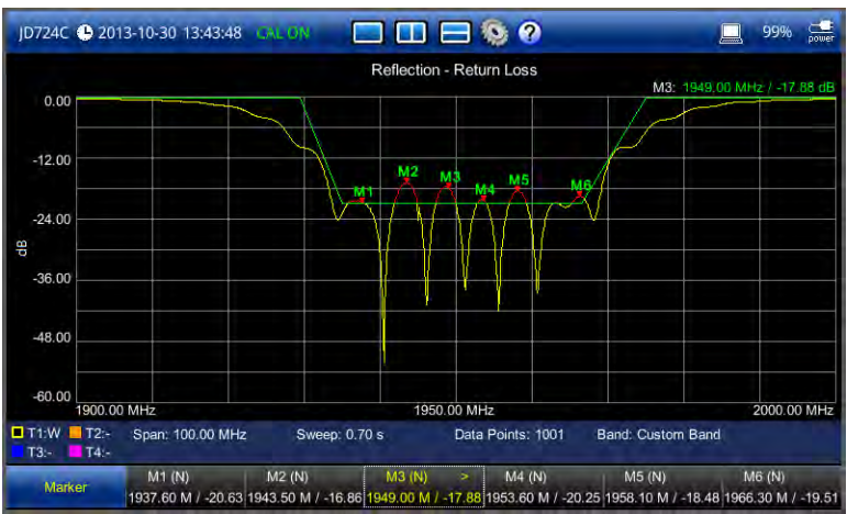
Figure 21 Reflection return loss measurement screen (zoom zones)
