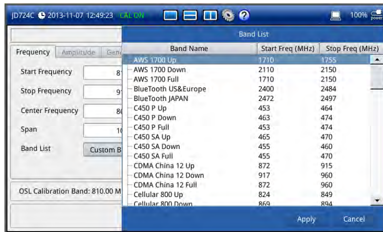
Figure 35 Band list window
