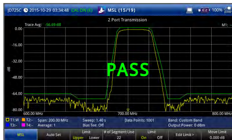
Figure 88 Task #15 “Limit Line - MSL” in 2 Port Transmission
