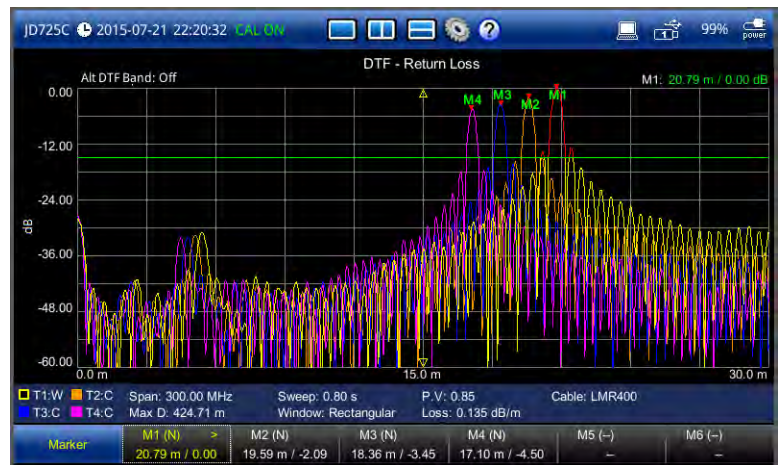
Figure 94 Trace overlay example
