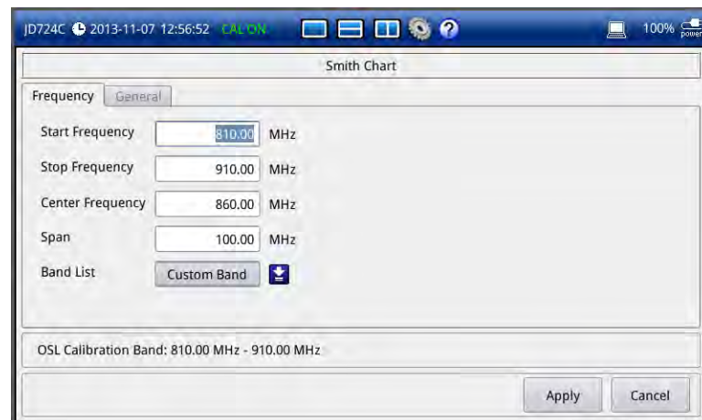
Figure 45 Frequency setup window for Smith chart measurements
