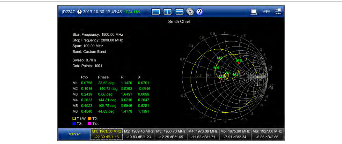
Figure 48 Smith chart measurement screen (single layout)
