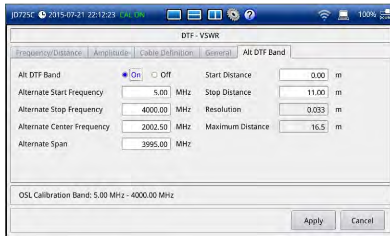
Figure 91 Alternate DTF band setting window
