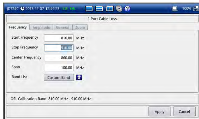
Figure 34 Frequency setup window for cable loss measurements
