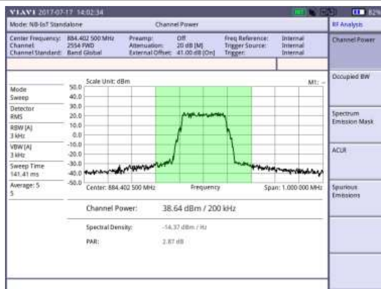
Figure 280 Channel power measurement with NB-IoT Standalone signal analyzer
