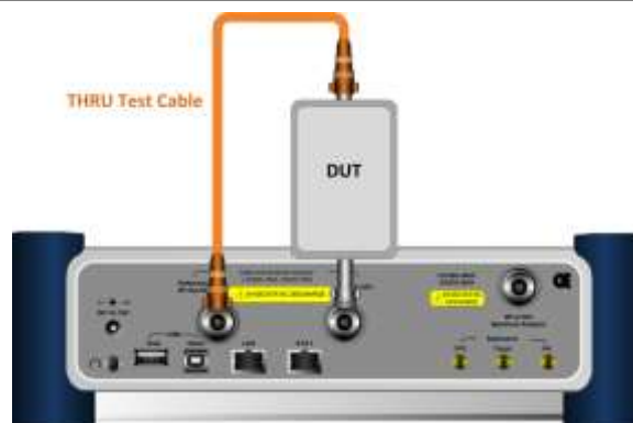
Figure 295 Connection for 2-port vector measurement
