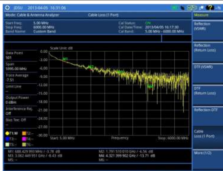
Figure 301 Cable loss (1 port) measurement
