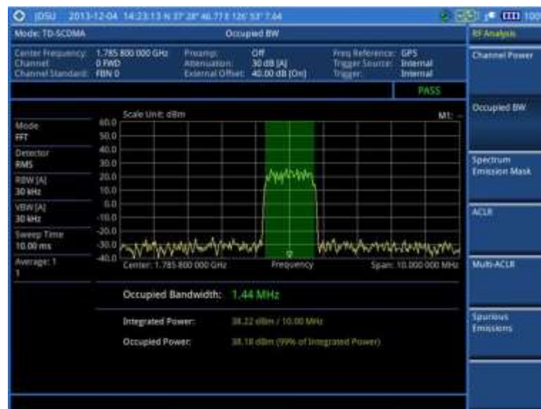
Figure 233 Occupied bandwidth measurement with TD-SCDMA signal analyzer
