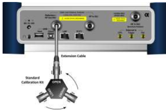
Figure 288 1-port calibration connection with mechanical Y-Cal kit
