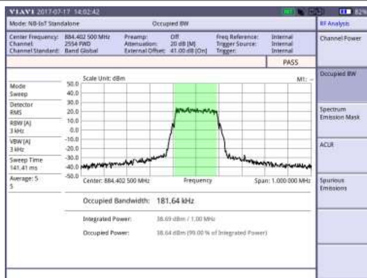
Figure 281 Occupied bandwidth measurement with NB-IoT Standalone signal analyzer
