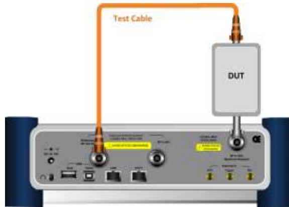
Figure 296 Connection for 2-port scalar measurement
