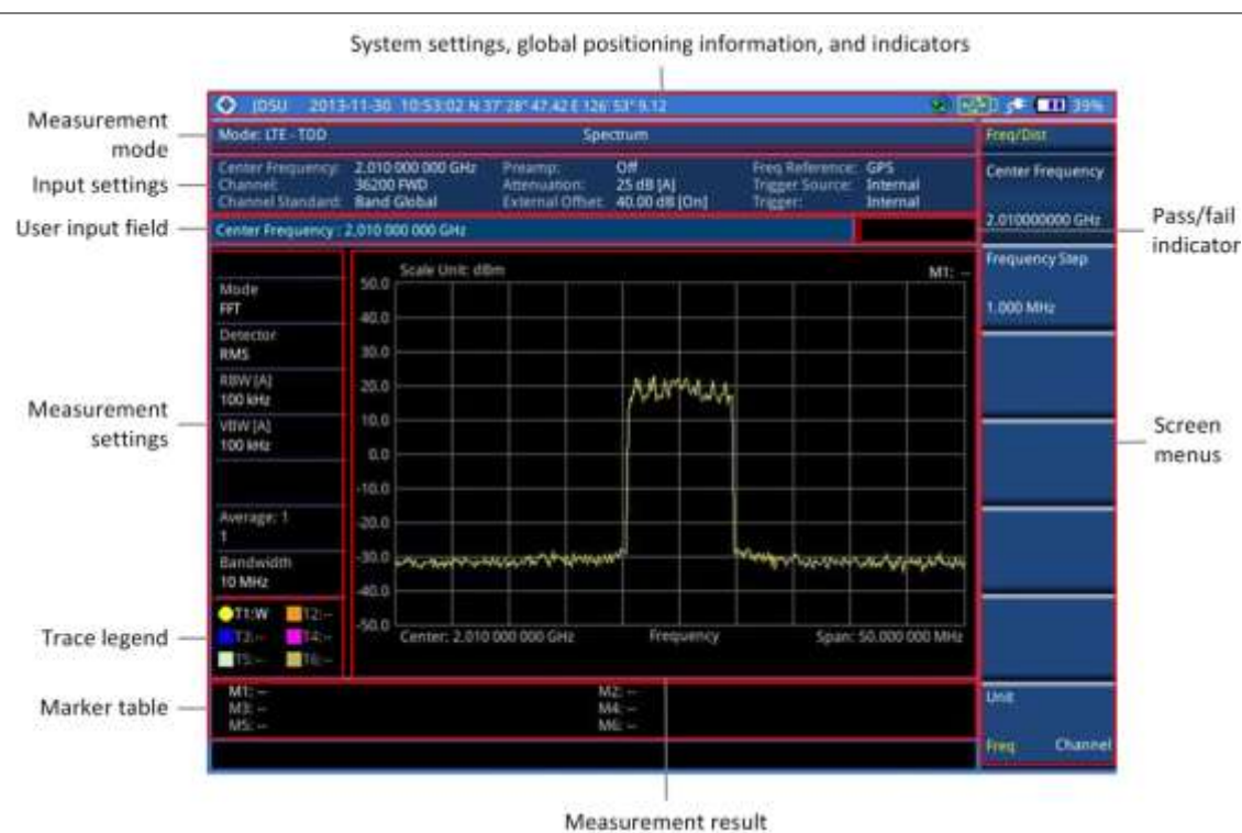
Figure 141 LTE - TDD signal analyzer measurement screen
