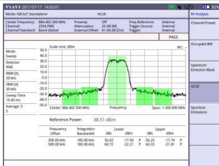
Figure 283 ACLR measurement with NB-IoT Standalone signal analyzer
