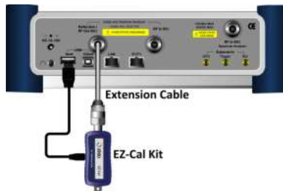
Figure 289 1-port calibration connection with electronic EZ-Cal kit
