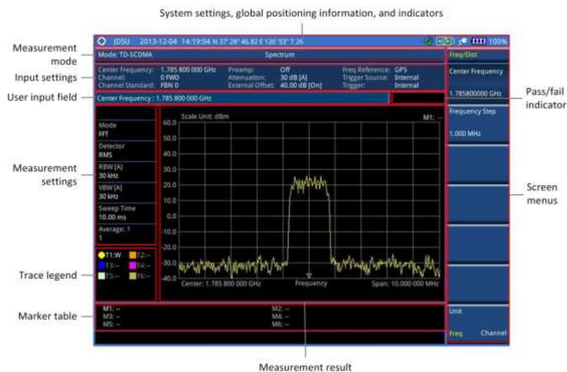
Figure 226 TD-SCDMA signal analyzer measurement screen
