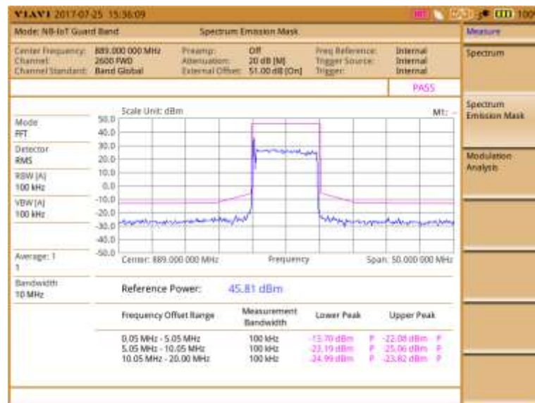
Figure 277 Spectrum Emission Mask measurement screen
