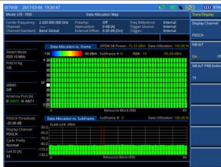
Figure 126 Data allocation map measurement with LTE - FDD signal analyzer (NB-IoT On)
