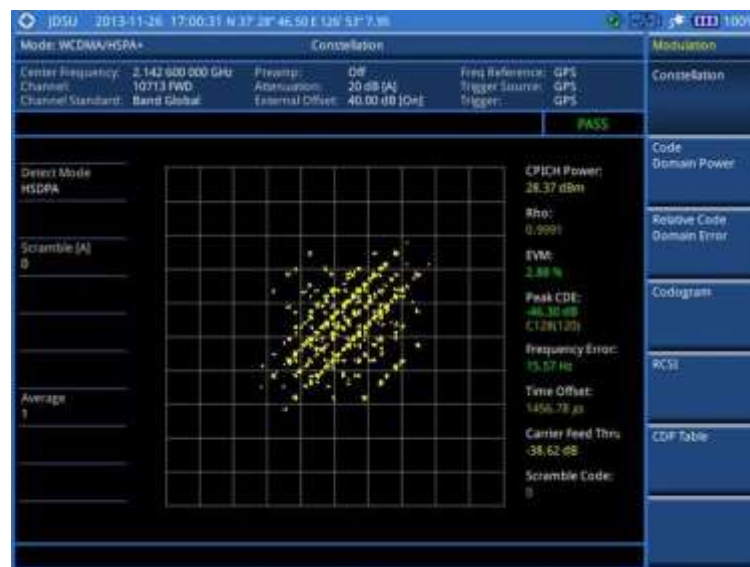
Figure 86 Constellation measurement with WCDMA/HSPA+ signal analyzer
