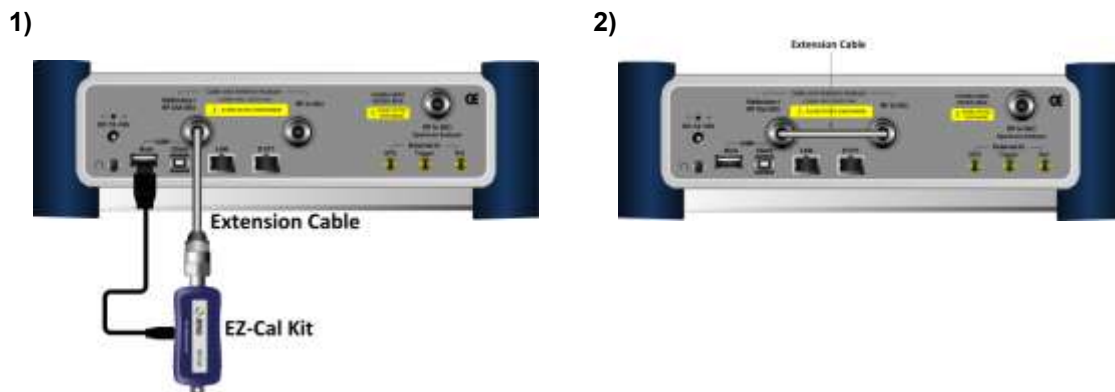
Figure 291 2-port calibration connection with EZ-Cal in vector measurements
