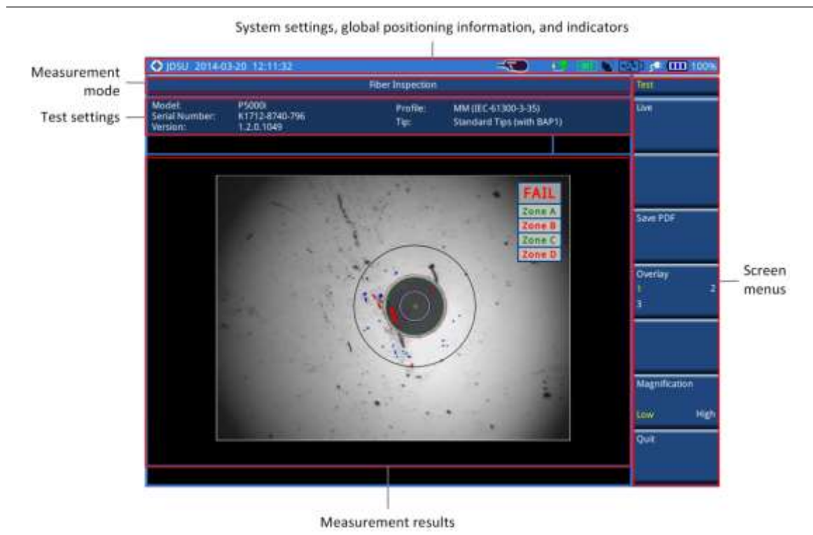
Figure 339 Fiber inspection screen
