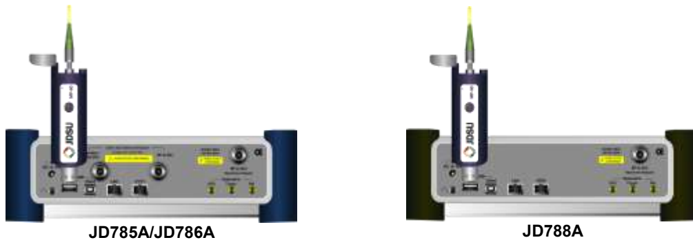
Figure 337 Optical power sensor connection
