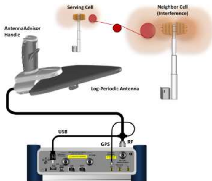
Figure 40 Connection using AntennaAdvisor handle and log-periodic antenna
