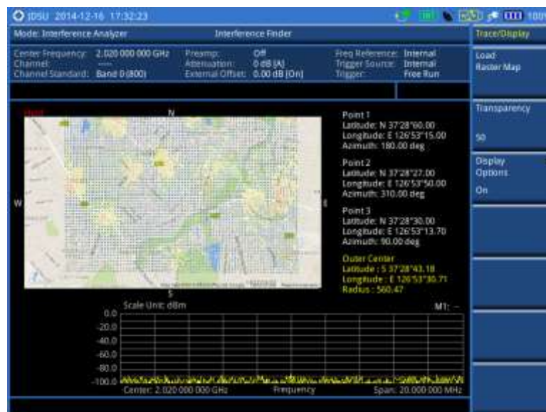
Figure 51 Raster image overlaid on the map in interference finder
