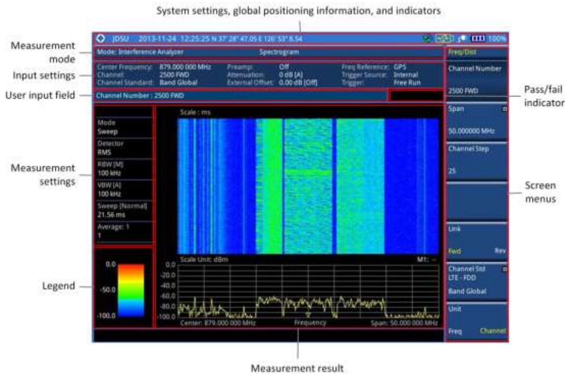
Figure 38 Interference measurement screen
