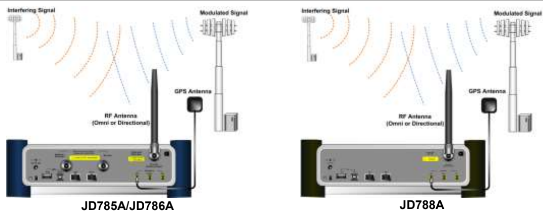
Figure 39 Interference measurement connection
