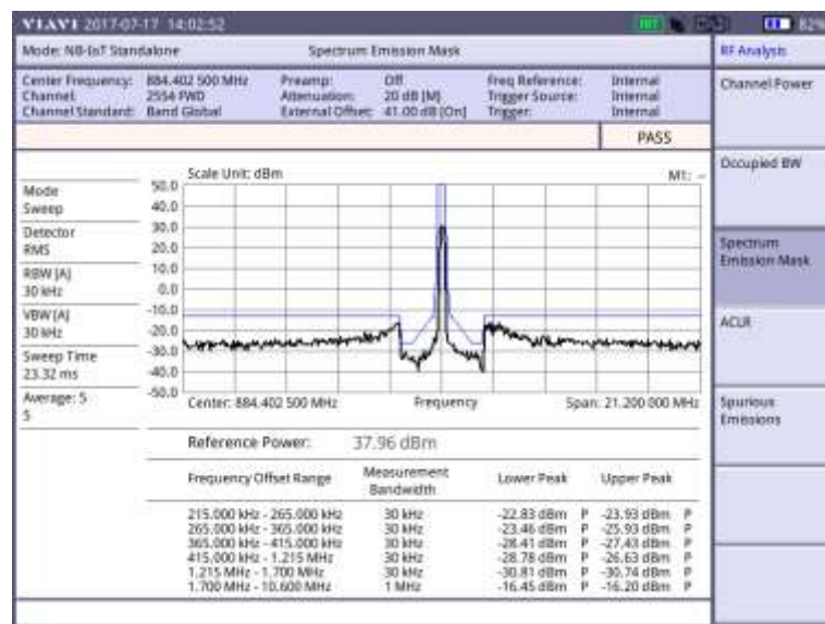
Figure 282 SEM measurement with NB-IoT Standalone signal analyzer
