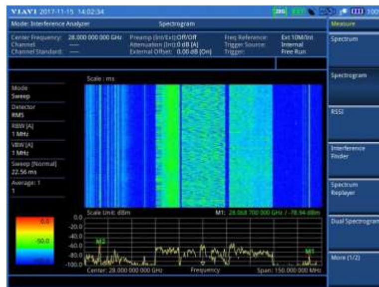
Figure 42 Interference measurement in spectrogram (on 28 GHz downconverter)
