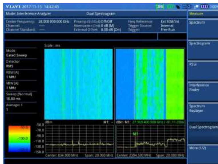
Figure 46 Interference measurement in dual spectrogram view (on 28 GHz downconverter)
