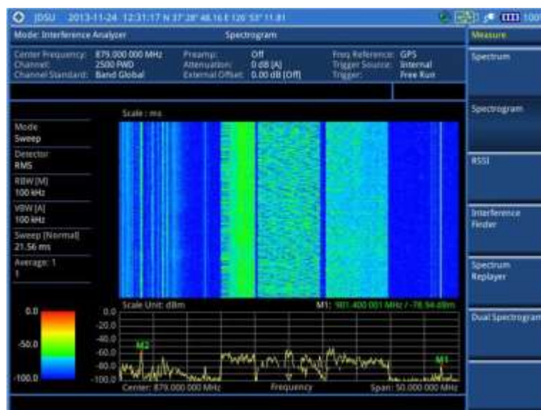
Figure 41 Interference measurement in spectrogram
