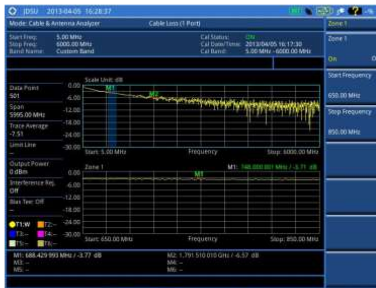
Figure 302 Cable loss (1 port) measurement with the zone enabled
