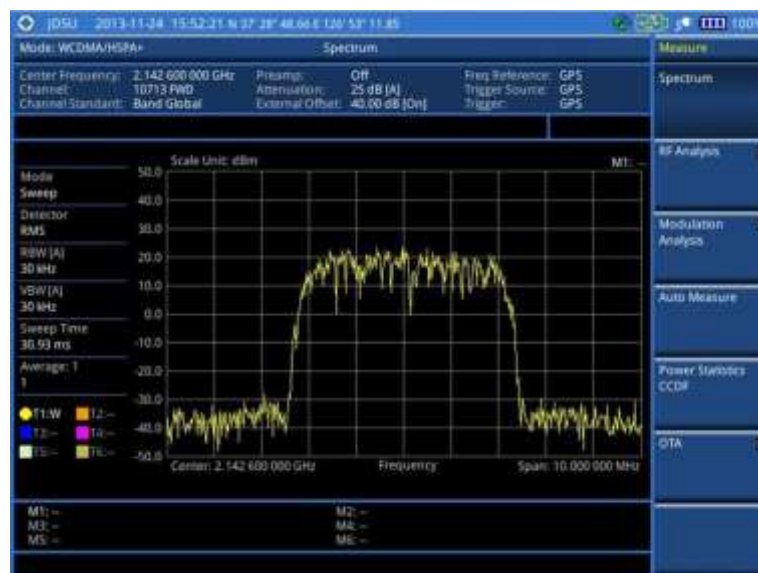
Figure 79 Spectrum measurement screen with WCDMA signal analyzer
