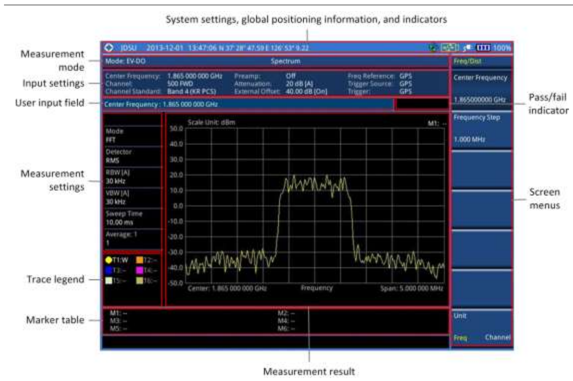
Figure 201 EV-DO signal analyzer measurement screen
