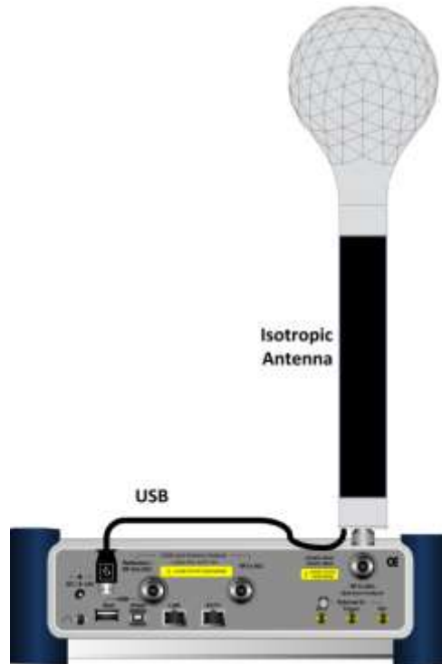
Figure 344 Connection using an isotropic antenna
