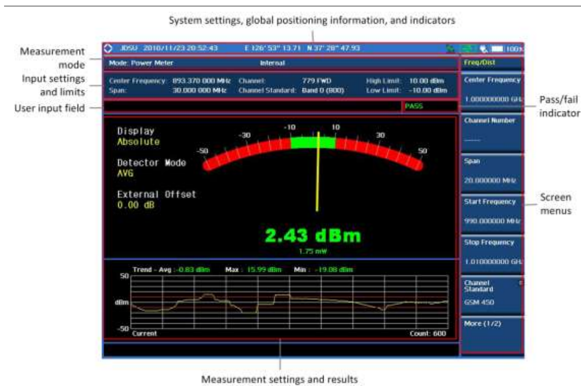
Figure 331 Power measurement screen
