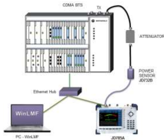
Figure 347 Using external power sensor
