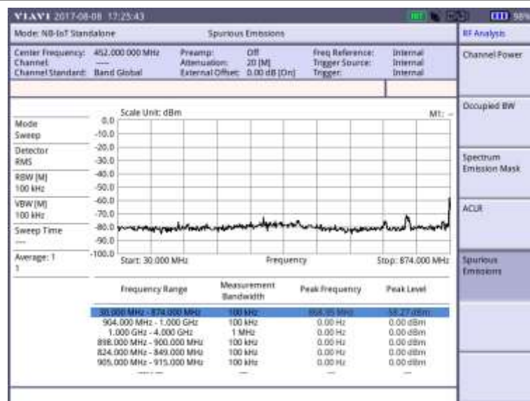
Figure 284 Spurious emissions measurement with NB-IoT Standalone signal analyzer
