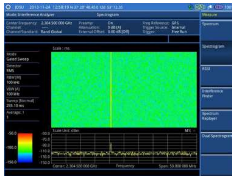
Figure 43 Interference measurement in spectrogram with gated sweep on
