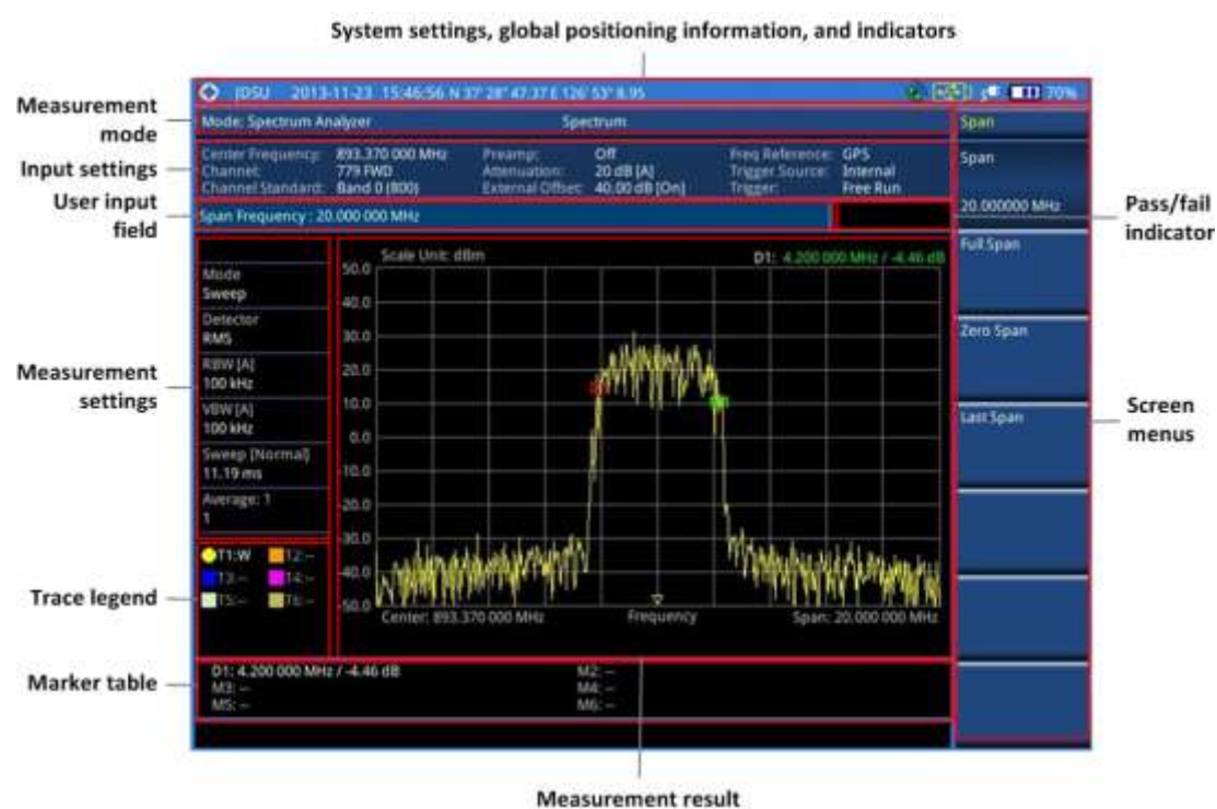
Figure 9 Spectrum measurement screen
