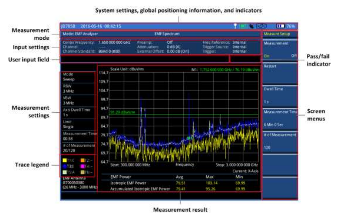
Figure 343 EMF Spectrum measurement screen
