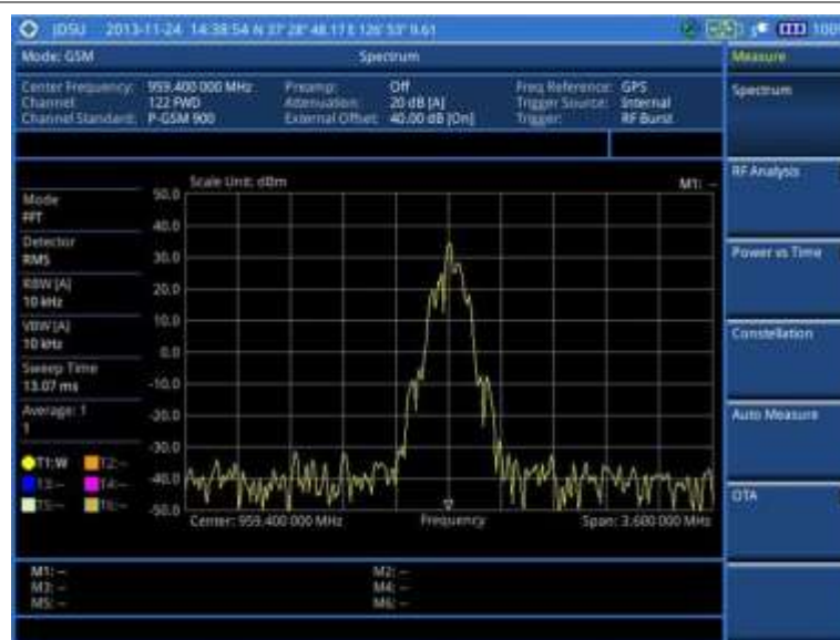
Figure 61 Spectrum measurement screen with GSM signal analyzer
