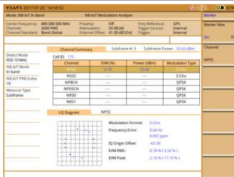
Figure 276 NB-IoT In Band Modulation Analysis measurement screen (Subframe 5-NPSS)
