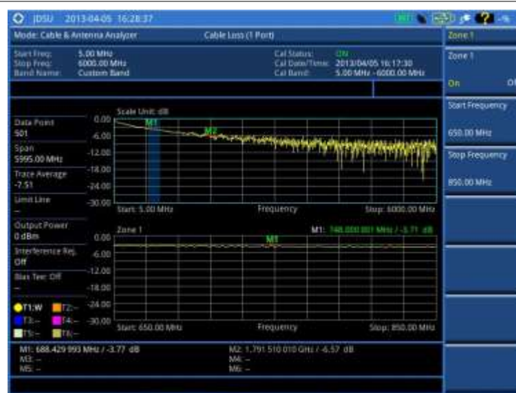
Figure 304 Cable loss (1 port) measurement with zoom
