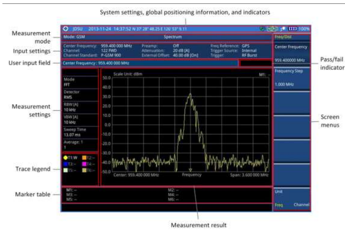
Figure 57 GSM signal analyzer measurement screen
