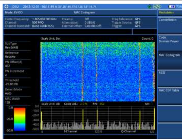
Figure 217 MAC Codogram in full view with EV-DO signal analyzer
