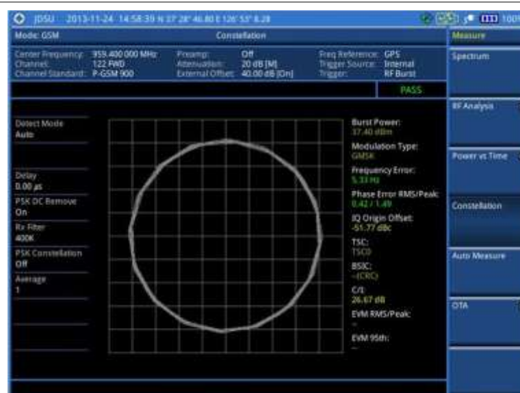
Figure 69 Constellation measurement with GSM signal analyzer
