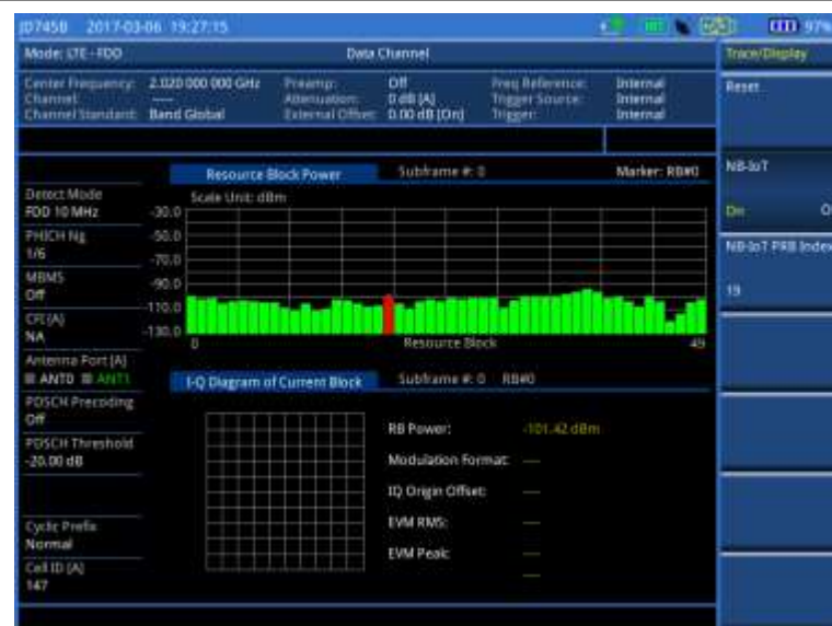
Figure 116 Data channel measurement with LTE - FDD signal analyzer (NB-IoT On)
