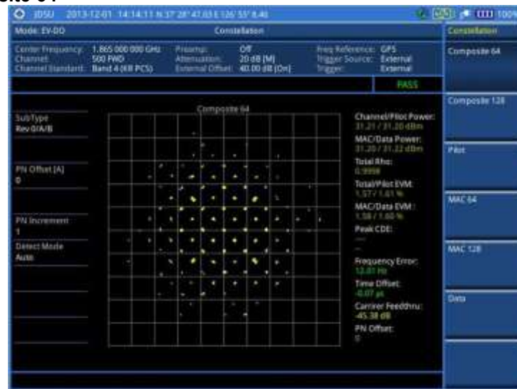
Figure 215 Constellation measurement with EV-DO signal analyzer
