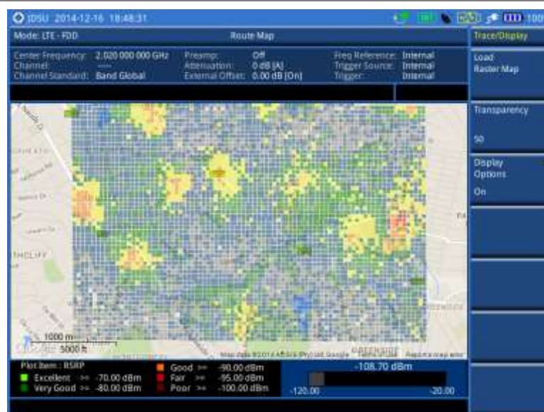
Figure 137 Raster image overlaid on the route map in LTE-FDD OTA signal analyzer
