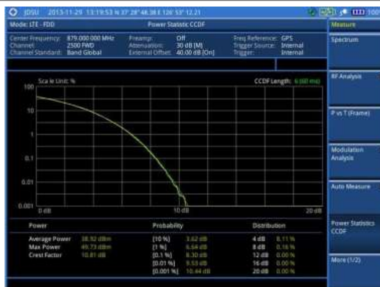
Figure 128 CCDF measurement with LTE - FDD signal analyzer
