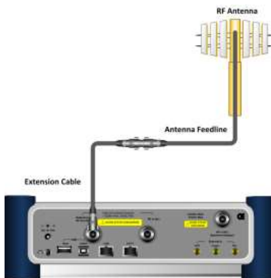
Figure 293 Connection for reflection measurement
