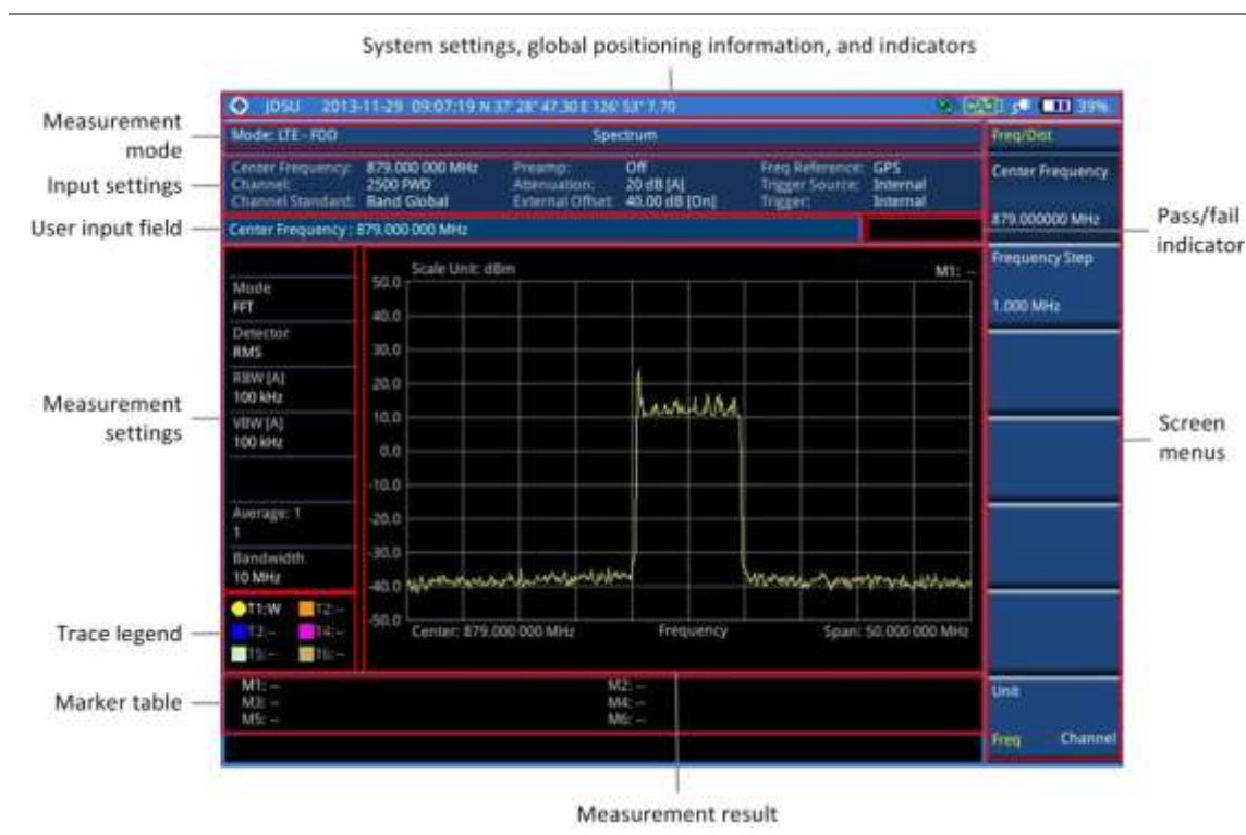
Figure 99 LTE - FDD signal analyzer measurement screen
