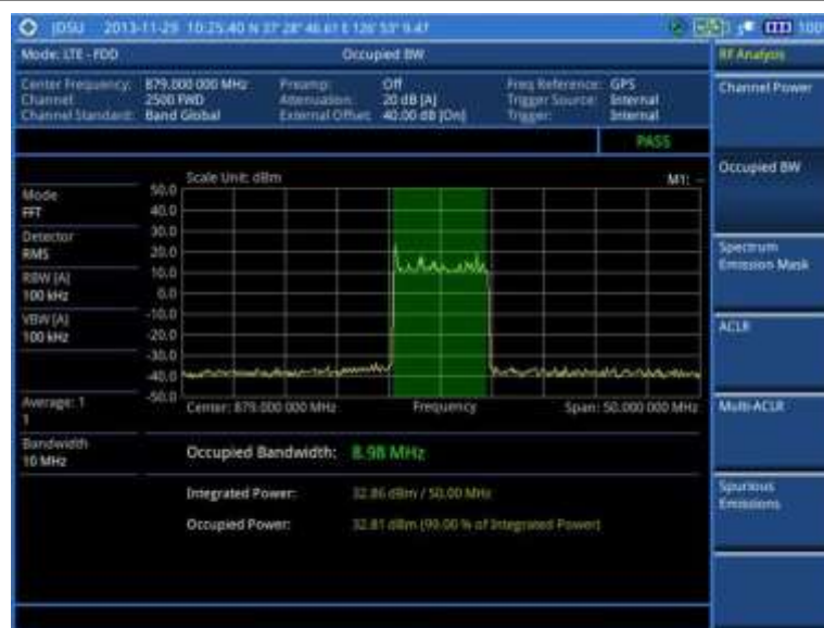
Figure 106 Occupied bandwidth measurement with LTE - FDD signal analyzer
