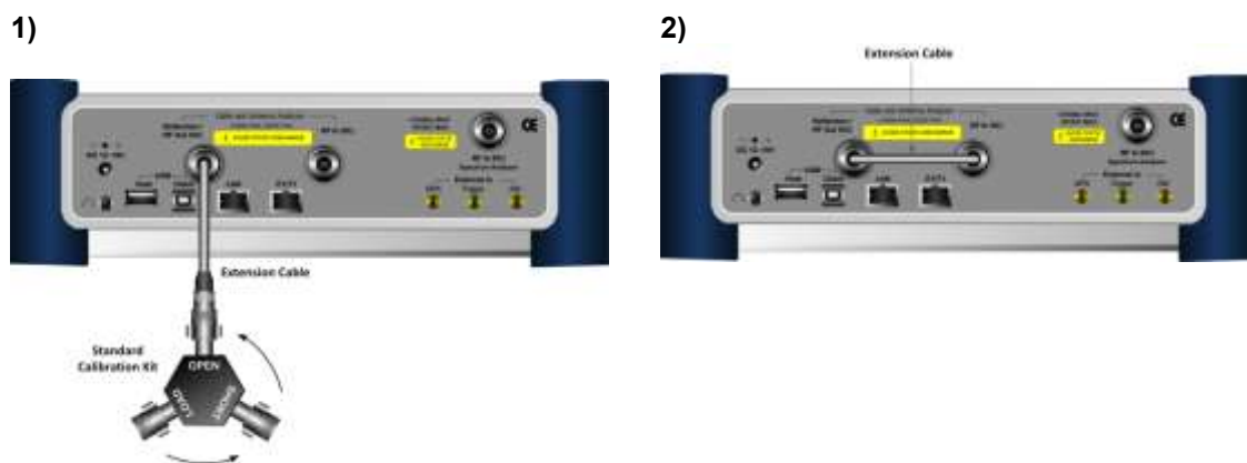
Figure 290 2-port calibration connection with Y-Cal in vector measurements
