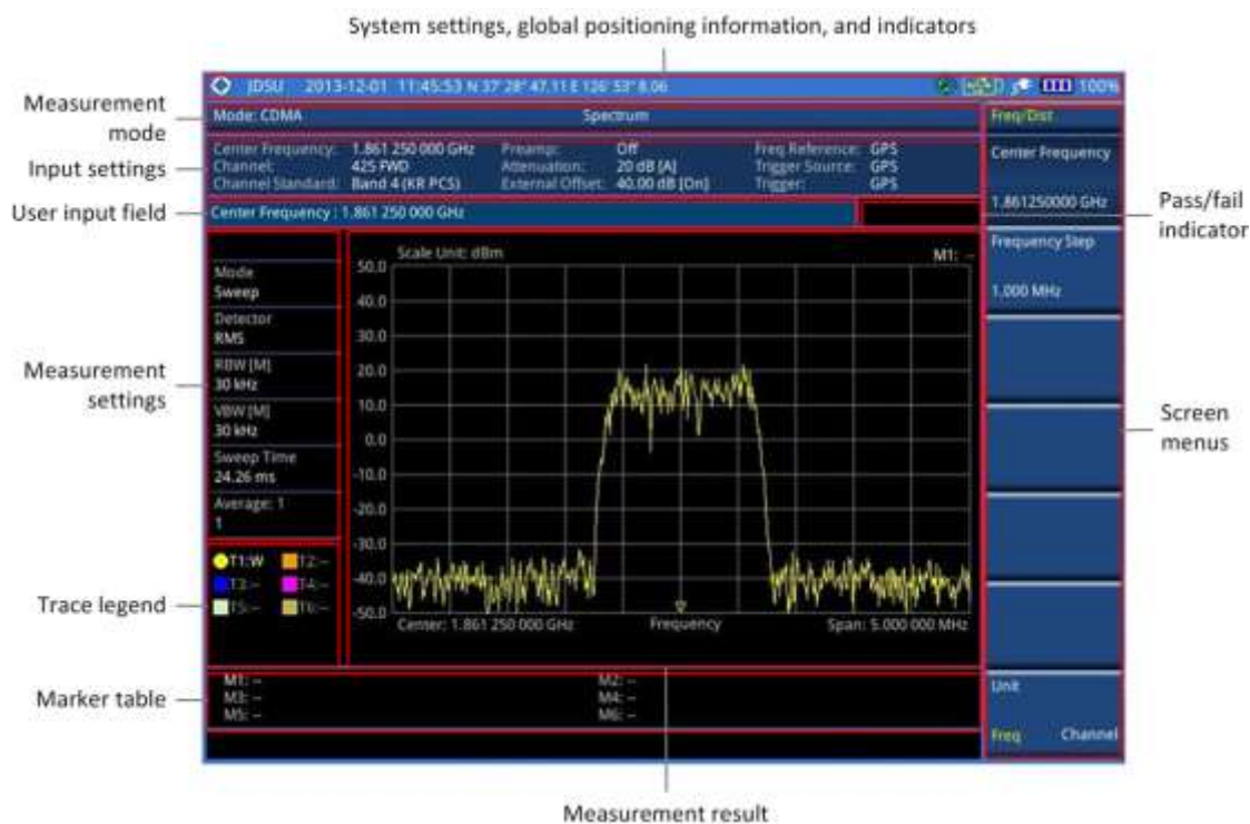
Figure 158 CDMA signal analyzer measurement screen
