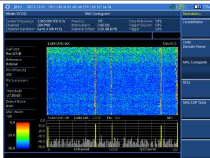
Figure 197 MAC Codogram in full view with EV-DO signal analyzer
