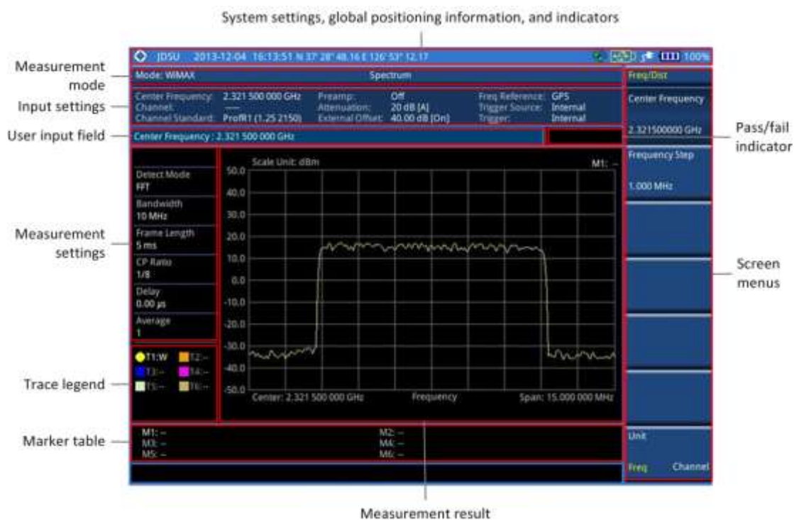
Figure 231 Mobile WiMAX signal analyzer measurement screen
