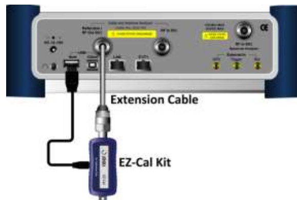
Figure 253 1-port calibration connection with electronic EZ-Cal kit
