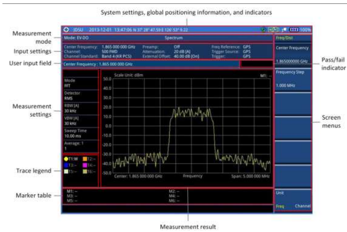
Figure 181 EV-DO signal analyzer measurement screen
