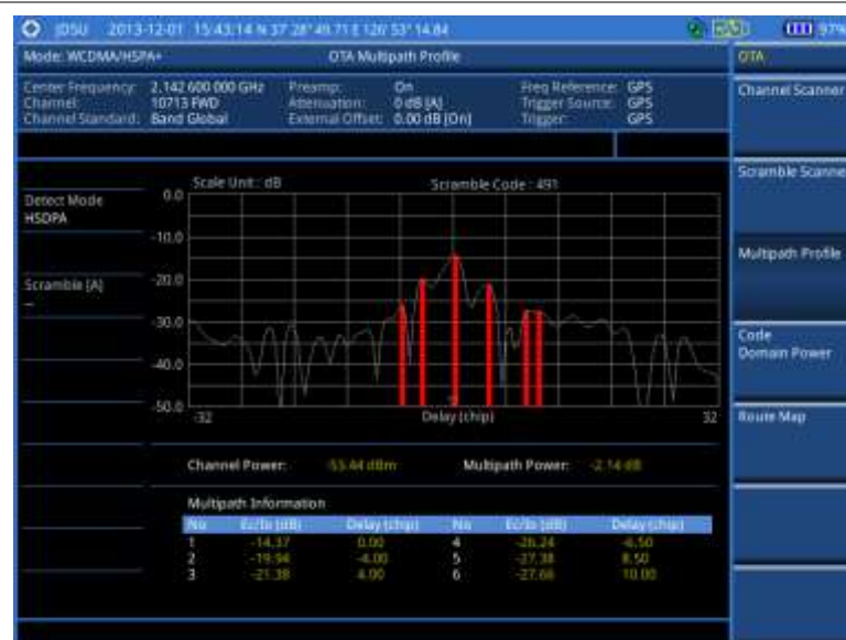
Figure 75 Multipath profile measurement with WCDMA/HSPA+ OTA signal analyzer
