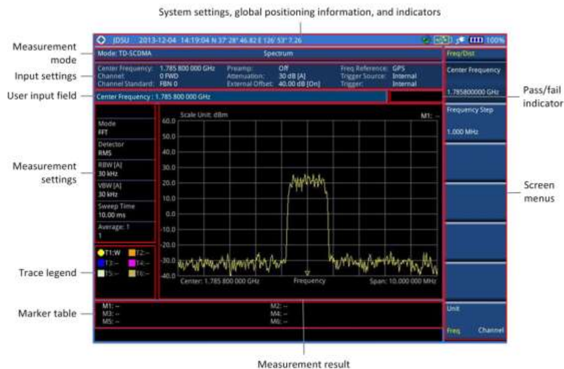
Figure 206 TD-SCDMA signal analyzer measurement screen
