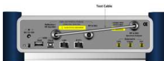
Figure 256 2-port calibration connection in Scalar measurements
