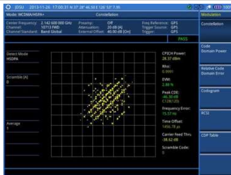
Figure 66 Constellation measurement with WCDMA/HSPA+ signal analyzer
