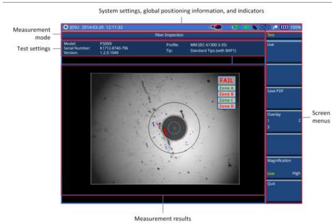
Figure 303 Fiber inspection screen
