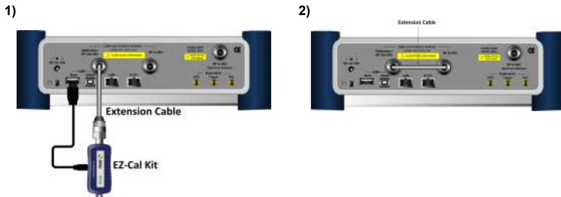
Figure 255 2-port calibration connection with EZ-Cal in vector measurements
