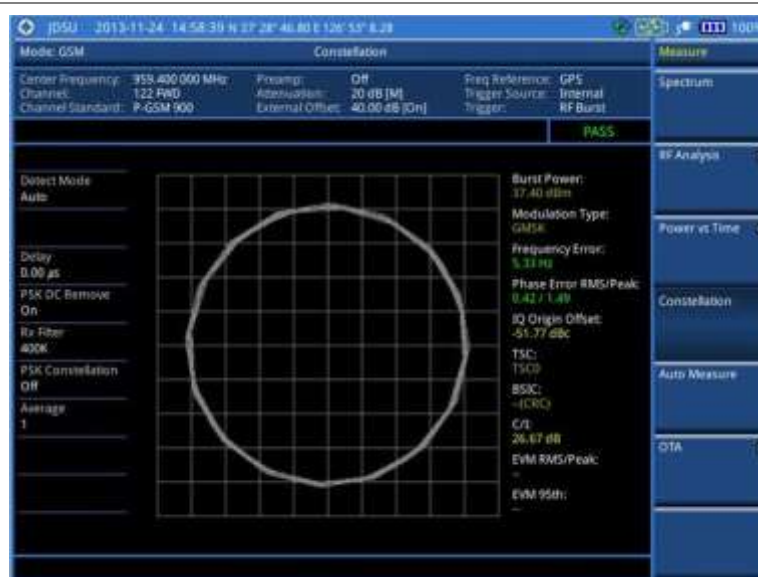
Figure 49 Constellation measurement with GSM signal analyzer
