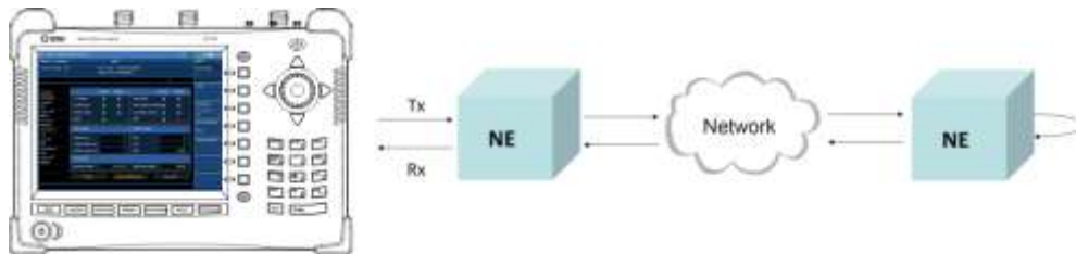
Figure 275 Error injection and measurement connection
