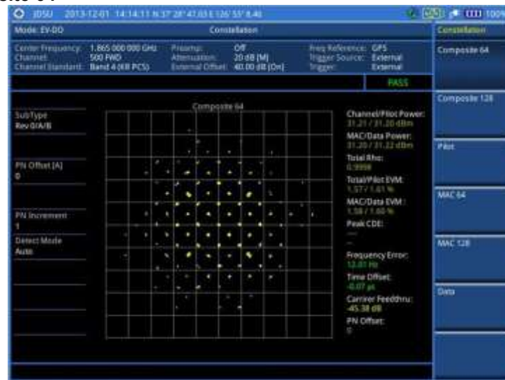
Figure 195 Constellation measurement with EV-DO signal analyzer
