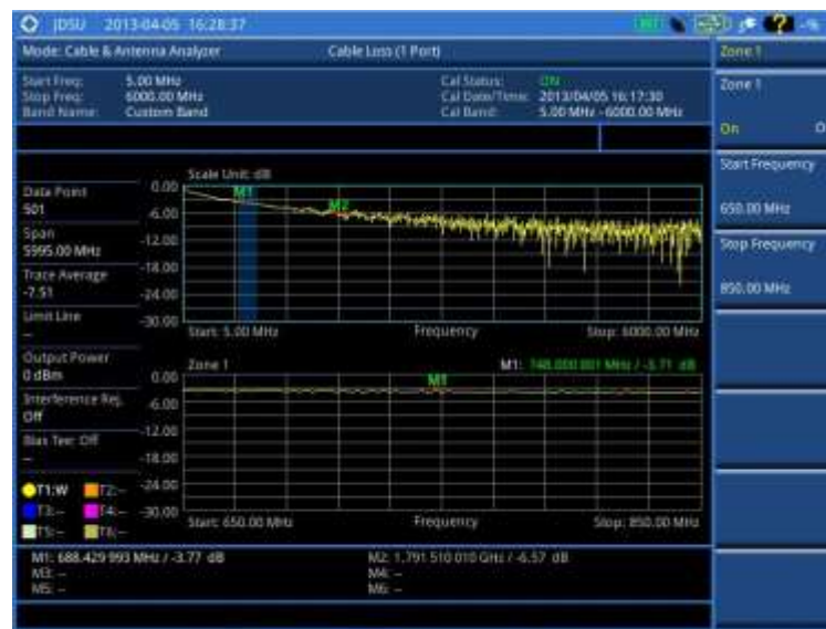
Figure 266 Cable loss (1 port) measurement with the zone enabled
