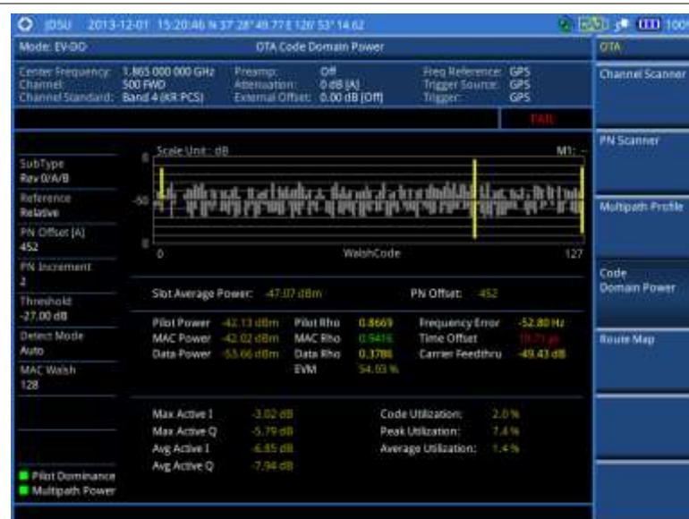
Figure 204 Code domain power measurement with EV-DO OTA signal analyzer
