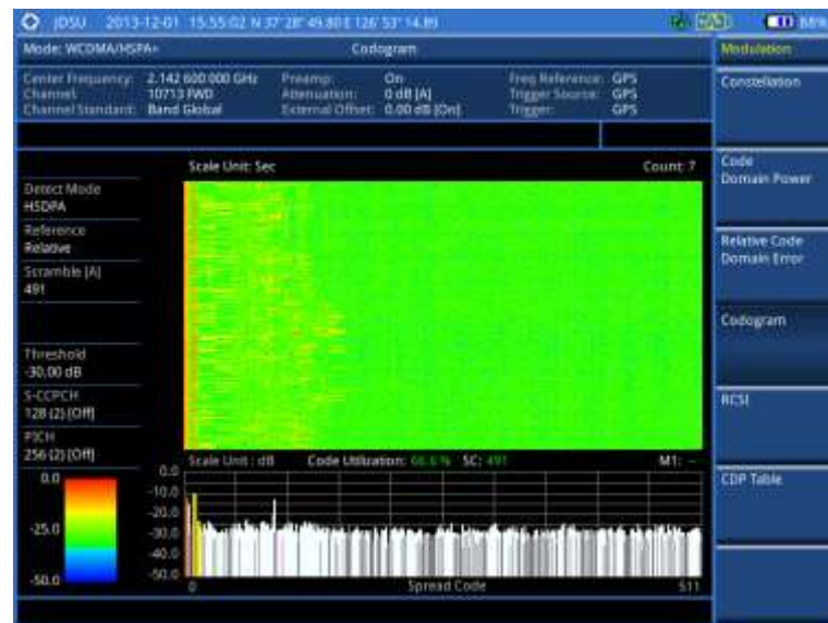
Figure 69 Codogram in full view with WCDMA/HSPA+ signal analyzer
