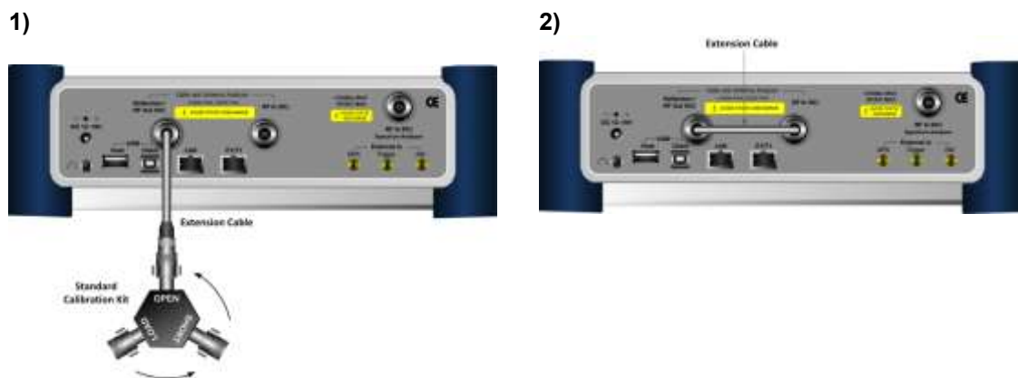
Figure 254 2-port calibration connection with Y-Cal in vector measurements
