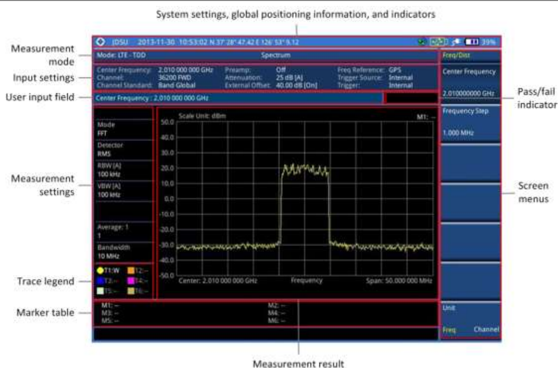
Figure 121 LTE - TDD signal analyzer measurement screen
