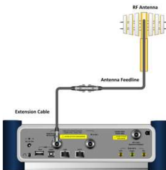
Figure 257 Connection for reflection measurement
