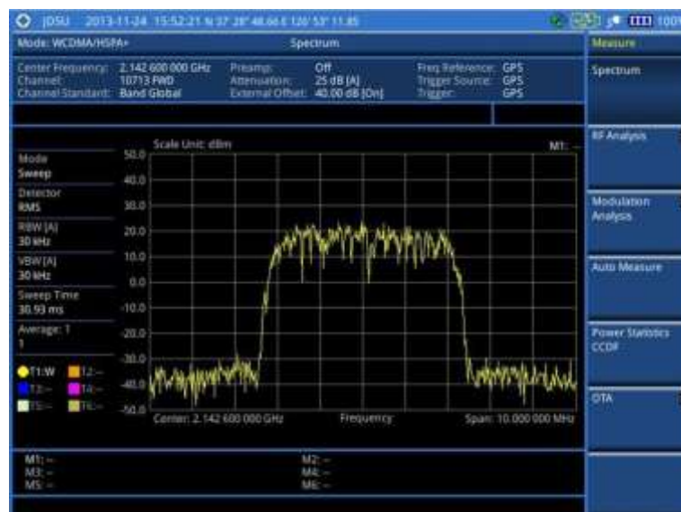
Figure 59 Spectrum measurement screen with WCDMA signal analyzer
