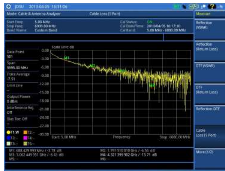
Figure 268 Cable loss (1 port) measurement with zoom
