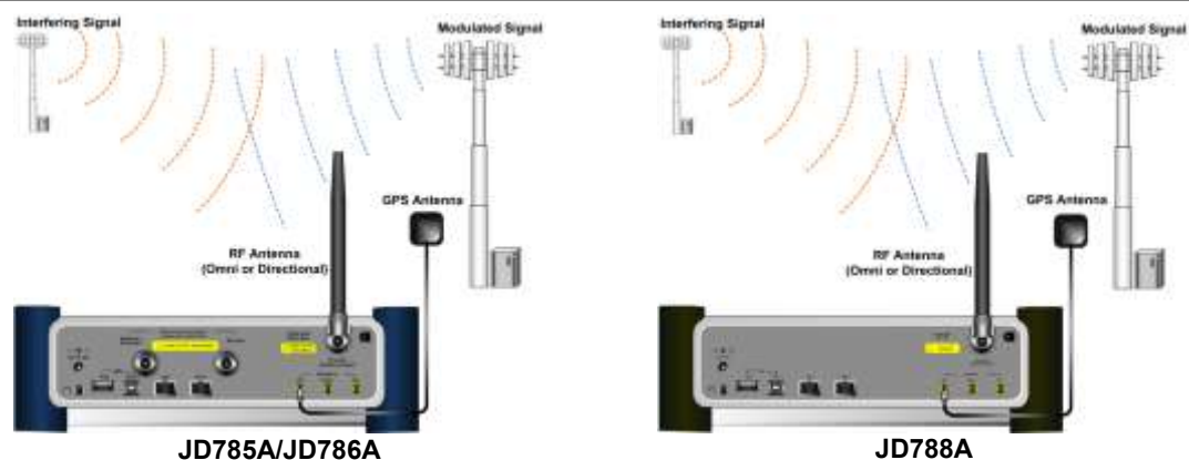
Figure 27 Interference measurement connection
