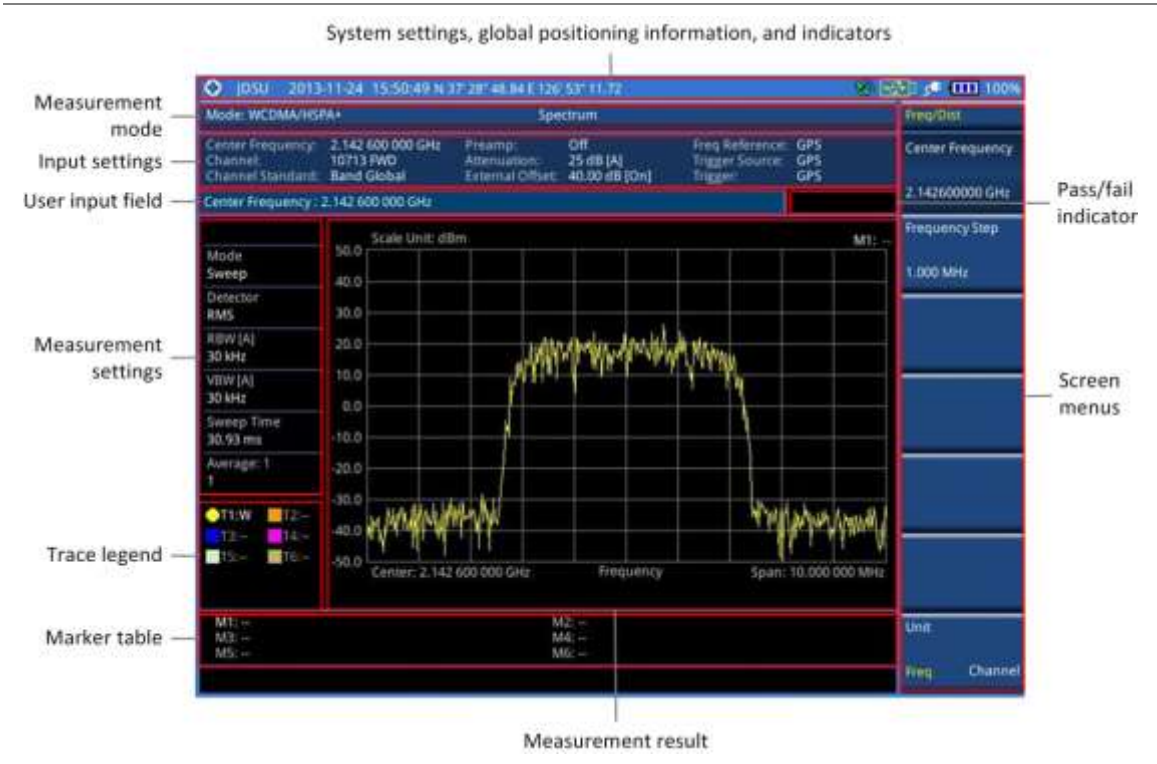
Figure 54 WCDMA/HSPA+ signal analyzer measurement screen
