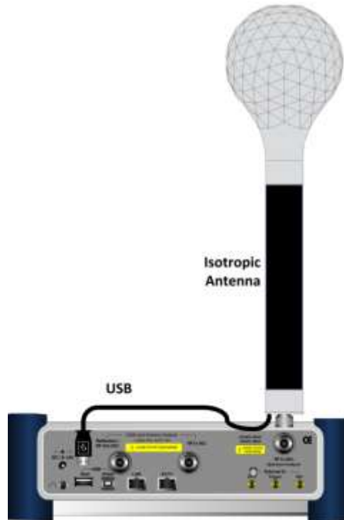
Figure 308 Connection using an isotropic antenna
