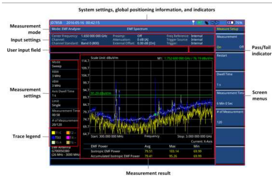
Figure 307 EMF Spectrum measurement screen
