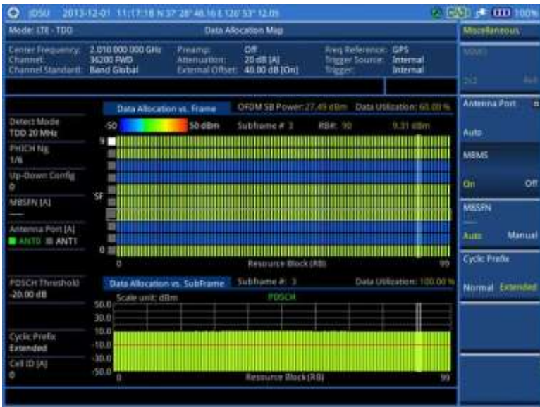
Figure 145 Data allocation map measurement with LTE - TDD signal analyzer (MBMS On)
