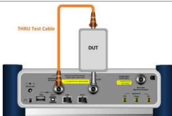
Figure 259 Connection for 2-port vector measurement
