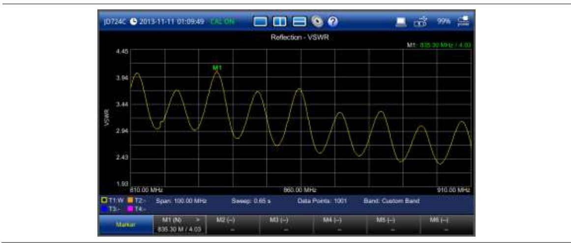
Figure 18 Reflection VSWR measurement screen (single layout)
