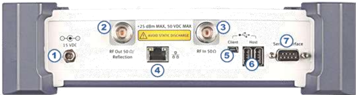
Figure 3 JD725C Top panel view
