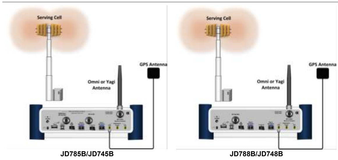
Figure 299 OTA connection
