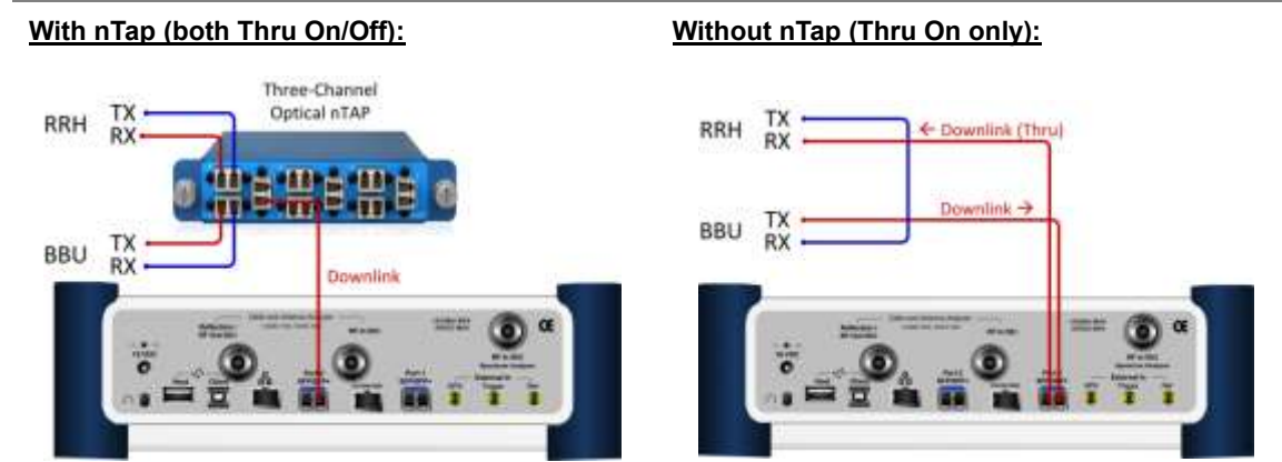
Figure 376 Connection diagram for downlink signal analysis
