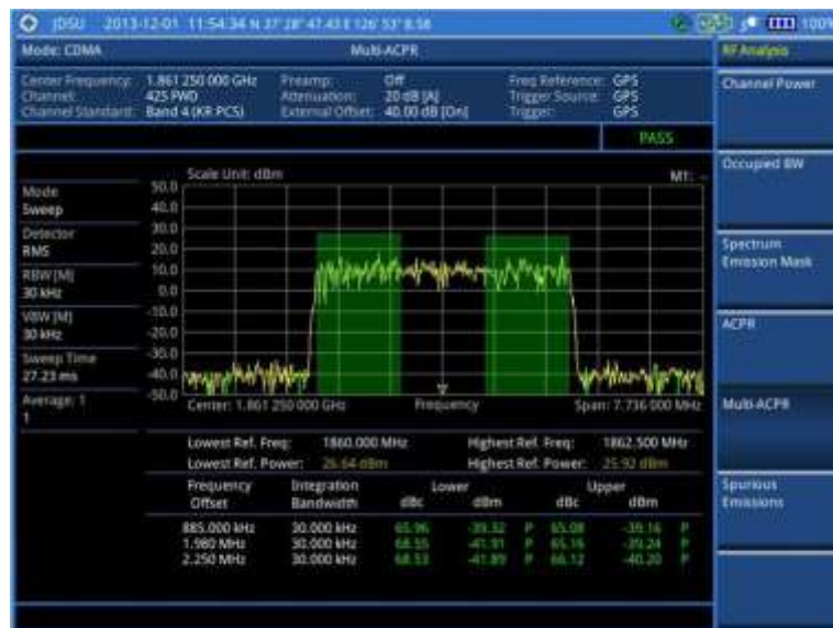
Figure 214 Multi-ACPR measurement with CDMA signal analyzer
