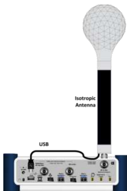
Figure 463 Connection using an isotropic antenna
