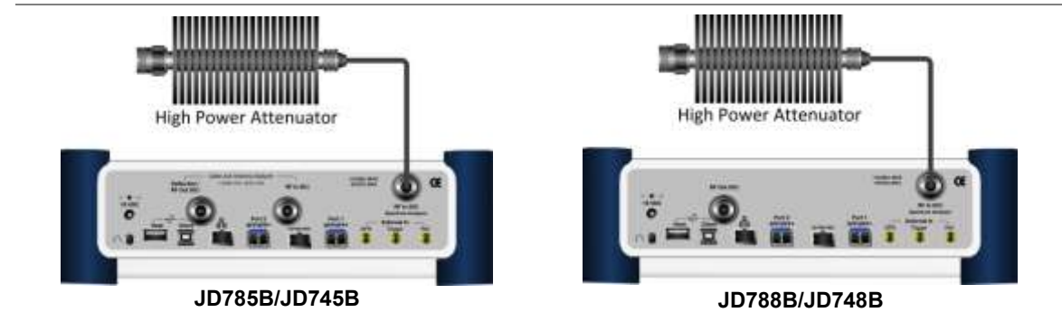
Figure 228 Direct connection
