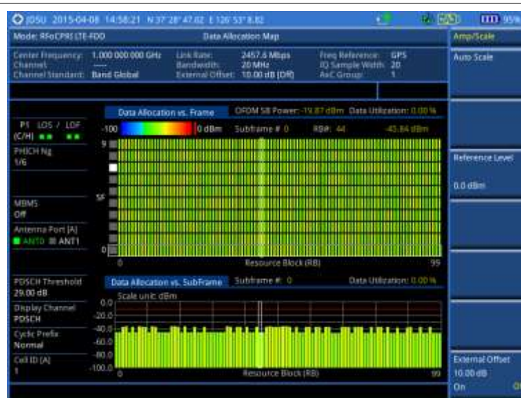
Figure 374 Data allocation map measurement with RFoCPRI LTE-FDD signal analyzer
