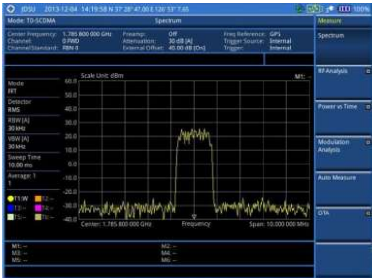
Figure 257 Spectrum measurement screen with TD-SCDMA signal analyzer
