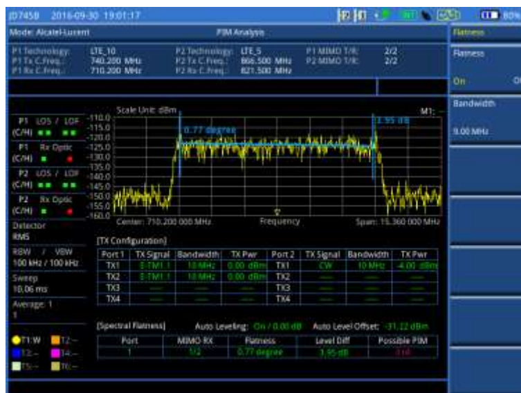
Figure 435 Example of Wideband Mode PIM analysis in Alcatel-Lucent BBU emulation
