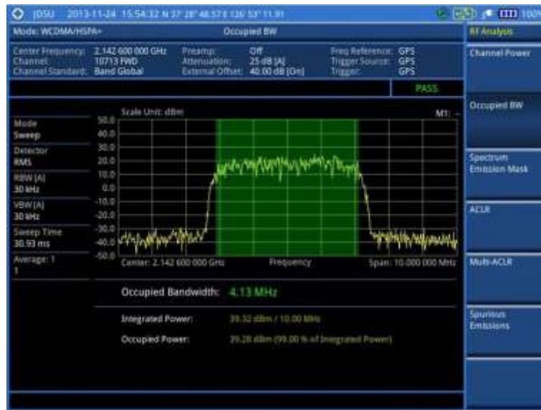
Figure 91 Occupied bandwidth measurement with WCDMA/HSPA+ signal analyzer
