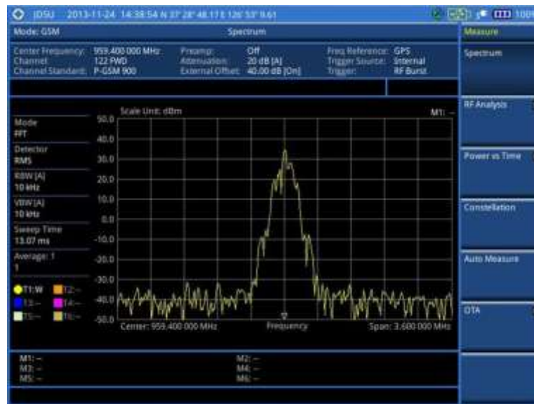
Figure 69 Spectrum measurement screen with GSM signal analyzer
