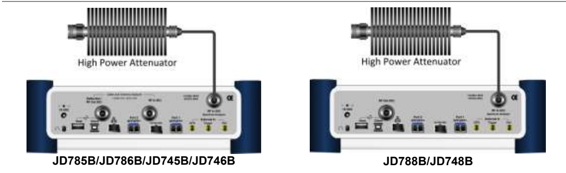
Figure 450 Direct connection
