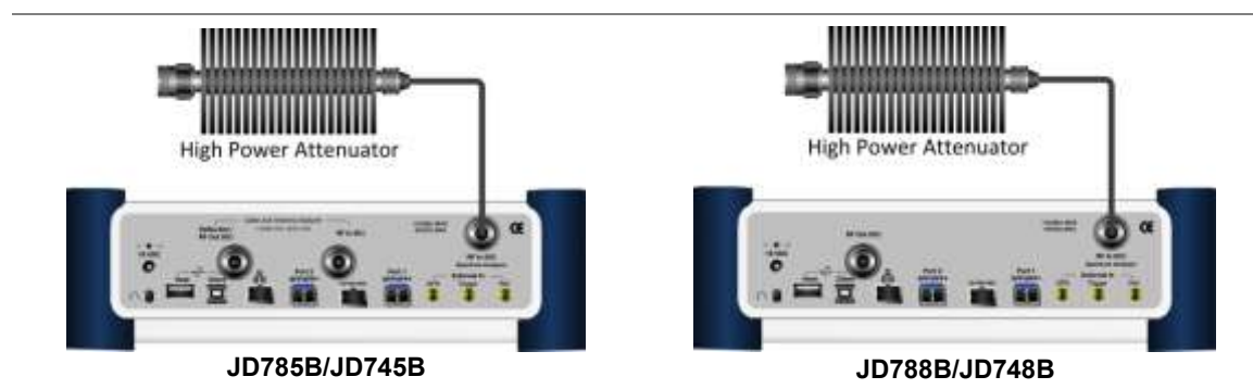
Figure 160 Direct connection
