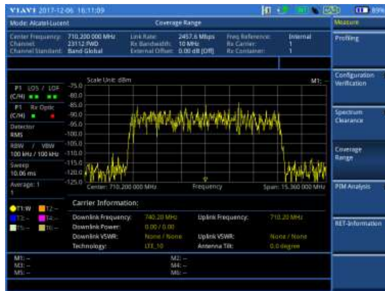
Figure 432 Example of coverage range in Alcatel-Lucent BBU emulation
