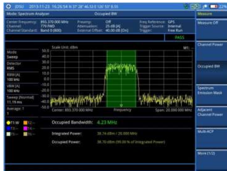
Figure 17 Occupied bandwidth measurement with spectrum analyzer
