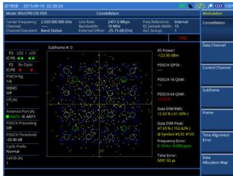
Figure 321 Constellation measurement with RFoCPRI LTE-FDD signal analyzer
