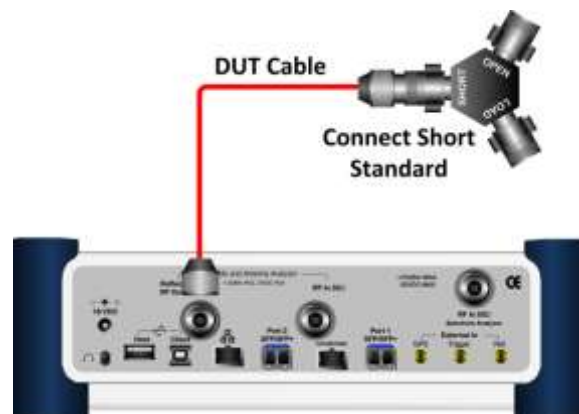
Figure 275 Connection for cable loss (1 port) measurement
