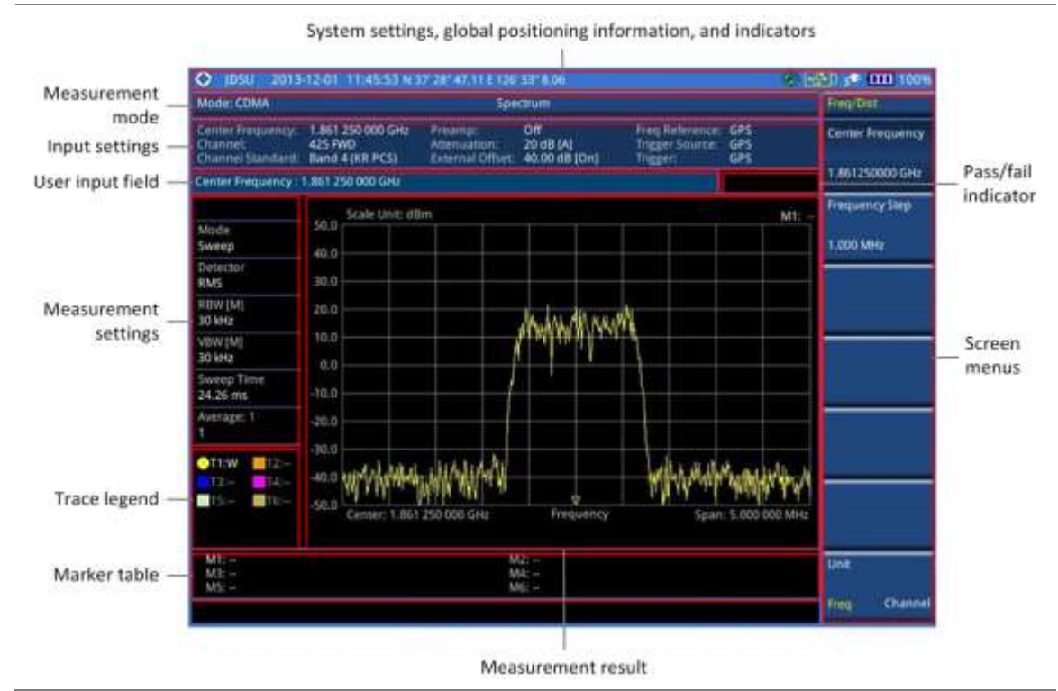
Figure 175 CDMA signal analyzer measurement screen
