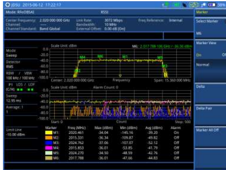
Figure 369 RFoBSAI interference measurement in RSSI
