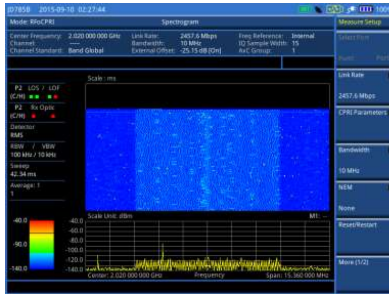
Figure 308 RFoCPRI interference measurement in spectrogram
