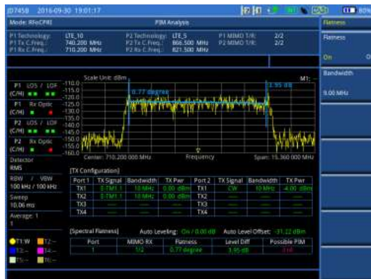
Figure 359 Example of Wideband Mode PIM analysis in BBU emulation
