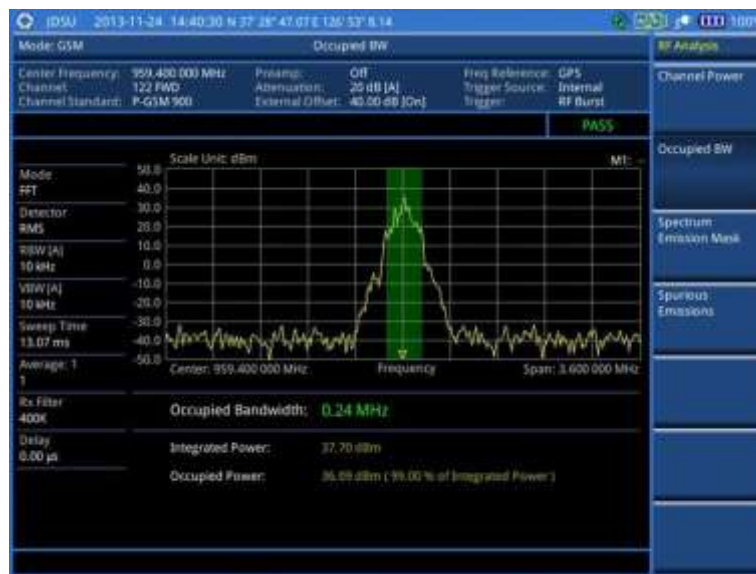
Figure 47 Occupied bandwidth measurement with GSM signal analyzer
