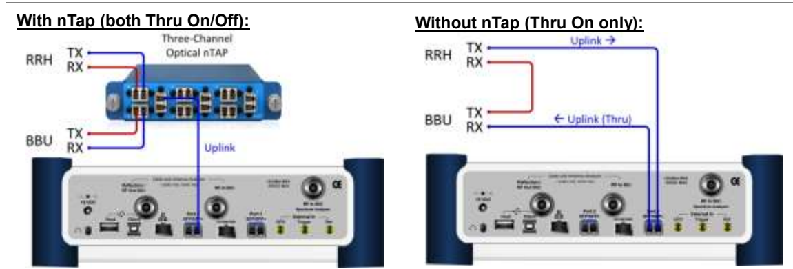
Figure 296 Connection diagram for interference analysis
