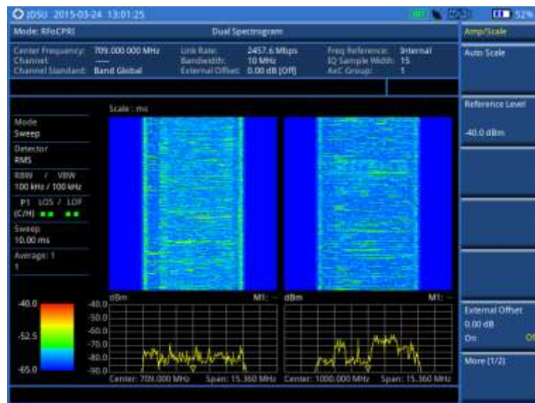
Figure 309 RFoCPRI dual spectrogram analysis
