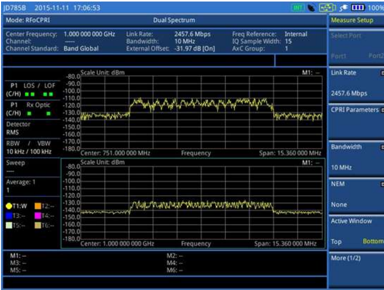
Figure 304 RFoCPRI dual spectrum with dual active trace off
