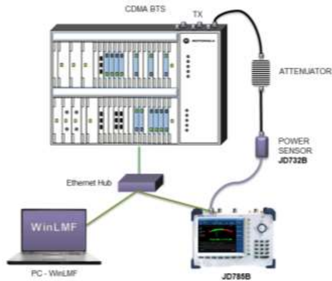
Figure 409 Using external power sensor
