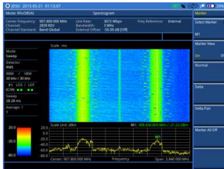
Figure 368 RFoBSAI interference measurement in spectrogram
