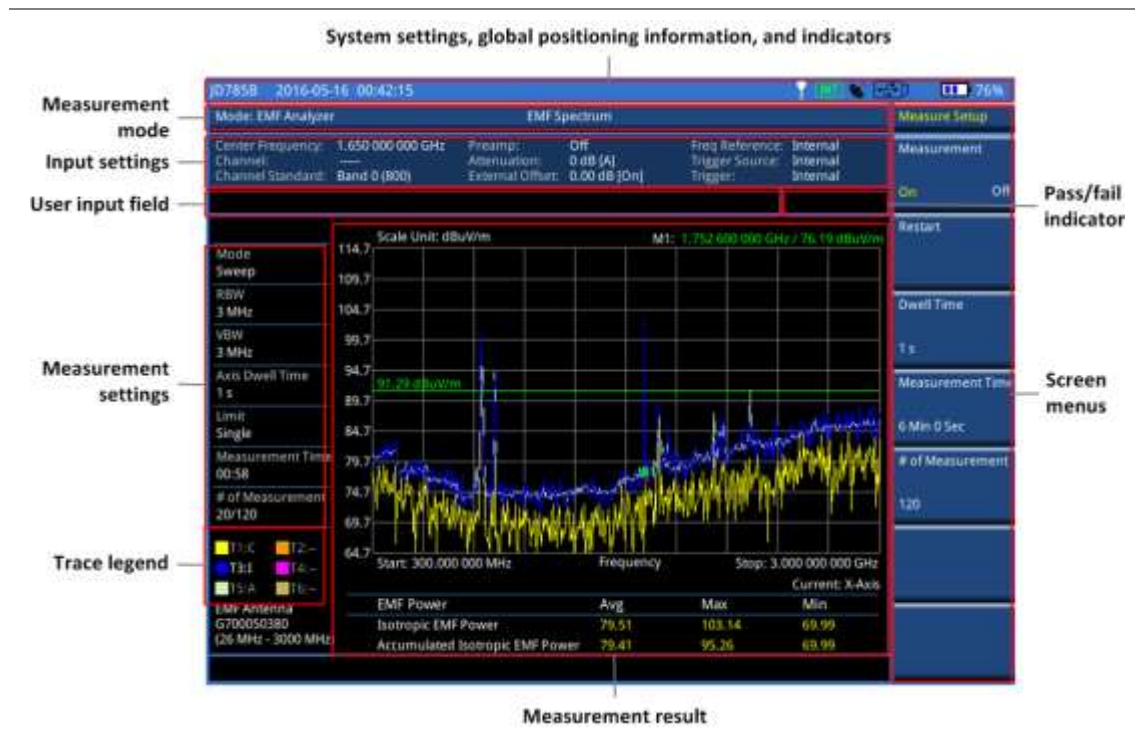
Figure 405 EMF Spectrum measurement screen
