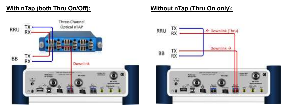
Figure 373 Connection diagram for downlink signal analysis
