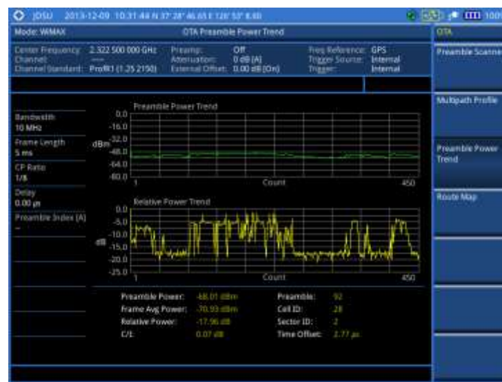
Figure 266 Preamble power trend with Mobile WiMAX OTA signal analyzer
