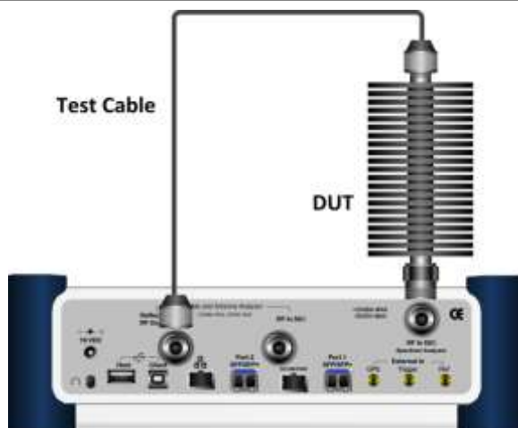
Figure 277 Connection for 2-port scalar measurement
