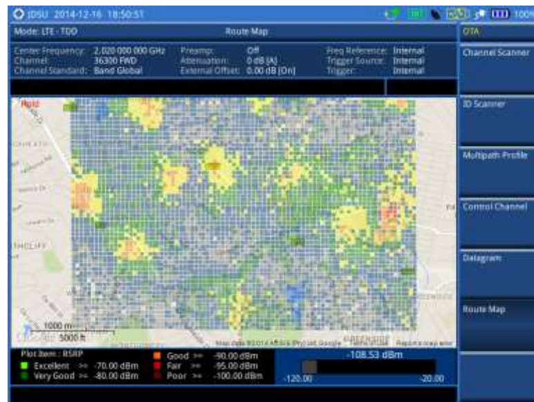
Figure 173 Raster image overlaid on the base map with LTE-TDD OTA signal analyzer
