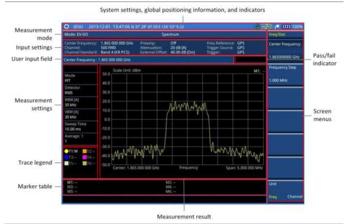
Figure 198 EV-DO signal analyzer measurement screen
