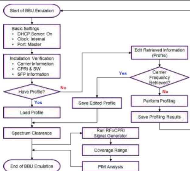
Figure 341 High-level workflow of BBU emulation
