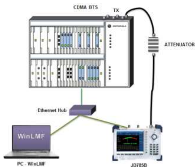
Figure 408 Using internal power sensor
