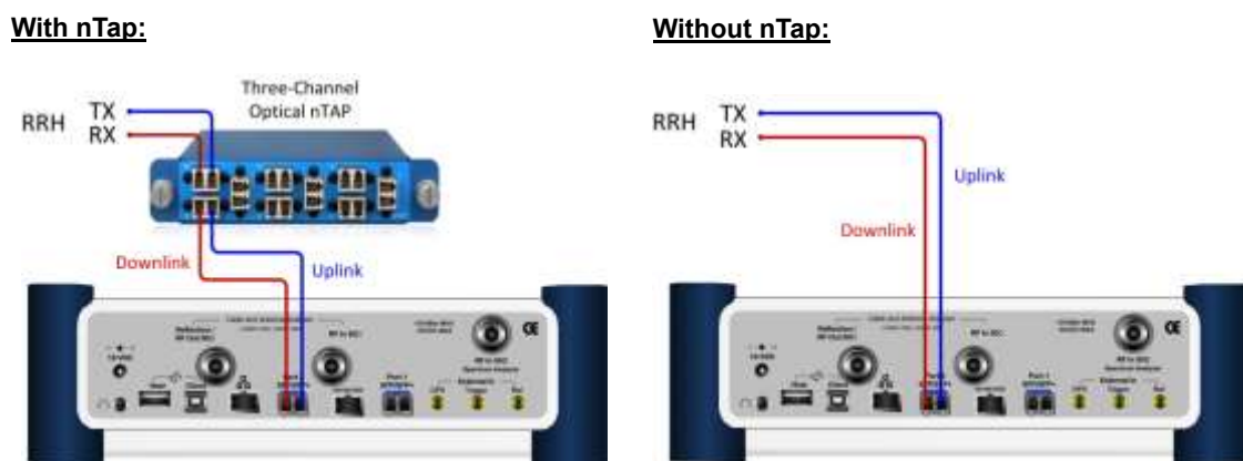
Figure 294 Connection diagram for Layer-2 BERT testing mode
