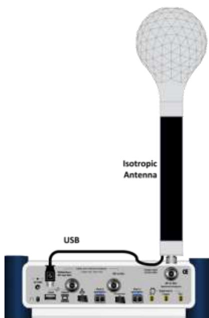
Figure 406 Connection using an isotropic antenna
