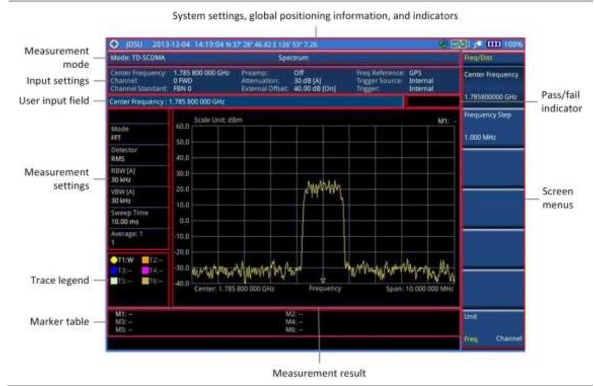
Figure 223 TD-SCDMA signal analyzer measurement screen
