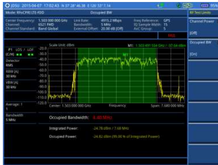
Figure 319 Occupied bandwidth measurement with RFoCPRI LTE-FDD signal analyzer
