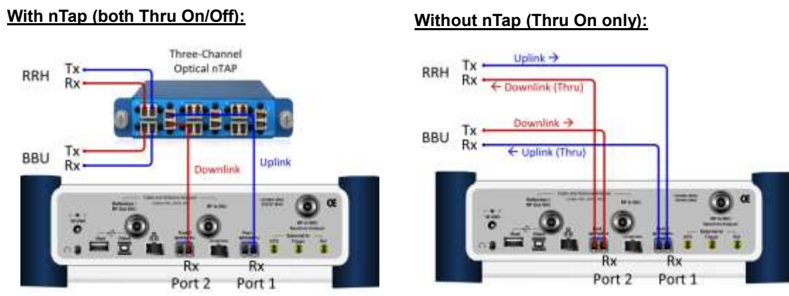
Figure 342 Thru connection diagram
