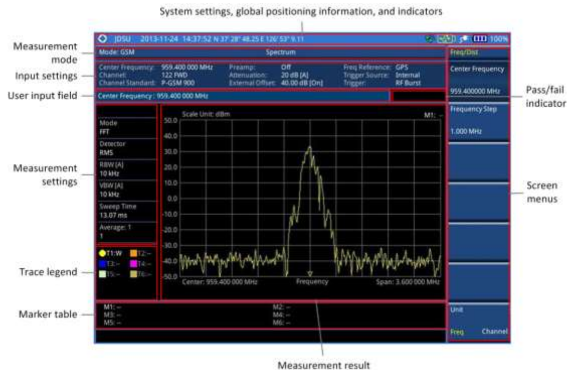
Figure 41 GSM signal analyzer measurement screen
