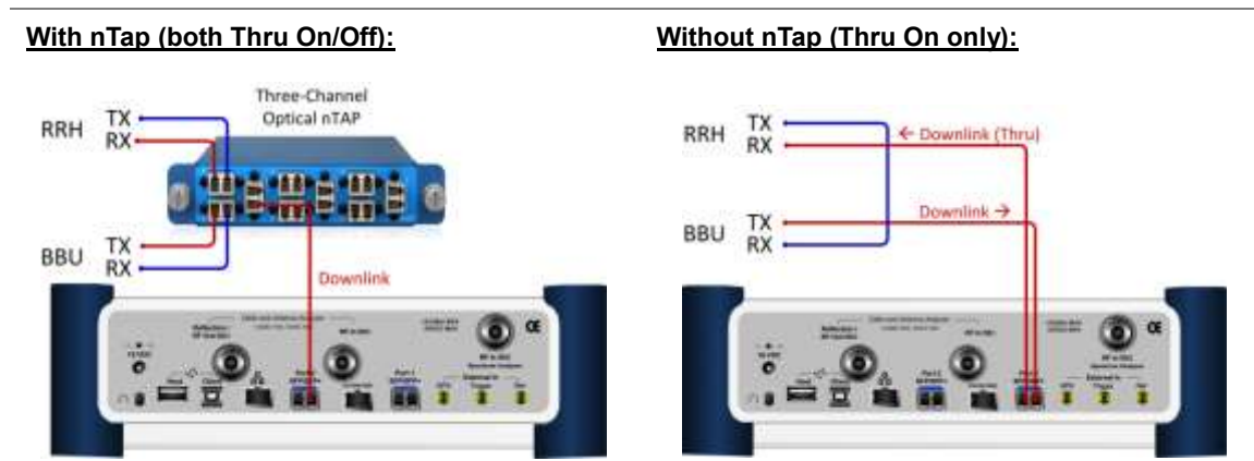
Figure 315 Connection diagram for downlink signal analysis
