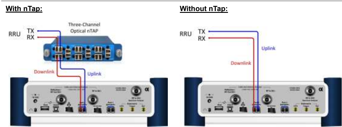
Figure 364 Connection diagram for Layer-2 term testing mode
