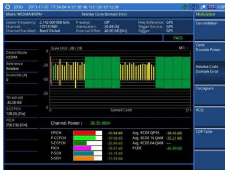
Figure 74 Relative code domain error with WCDMA/HSPA+ signal analyzer
