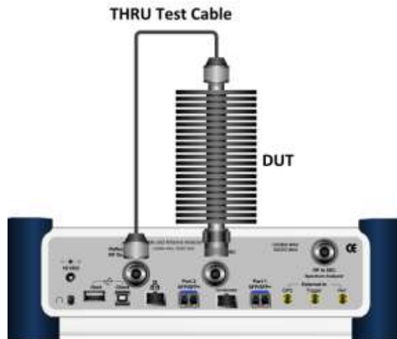
Figure 276 Connection for 2-port vector measurement
