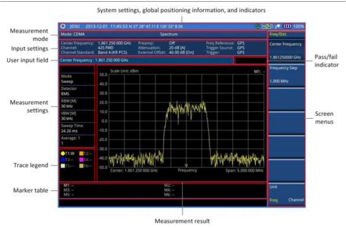
Figure 175 CDMA signal analyzer measurement screen
