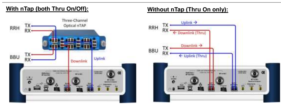
Figure 290 Connection diagram for Layer-2 monitoring mode
