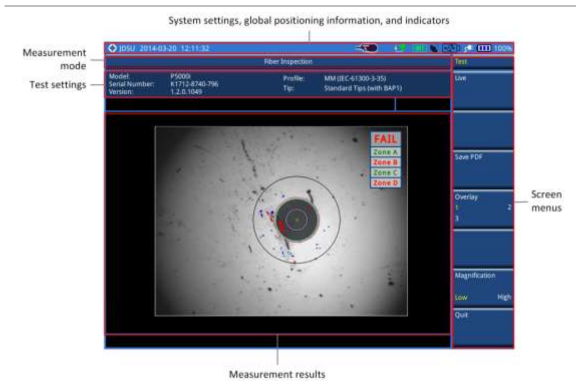
Figure 399 Fiber inspection screen
