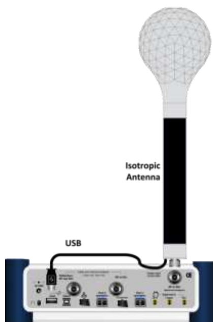
Figure 404 Connection using an isotropic antenna
