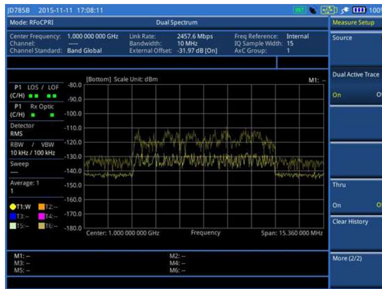
Figure 303 RFoCPRI dual spectrum with dual active trace on
