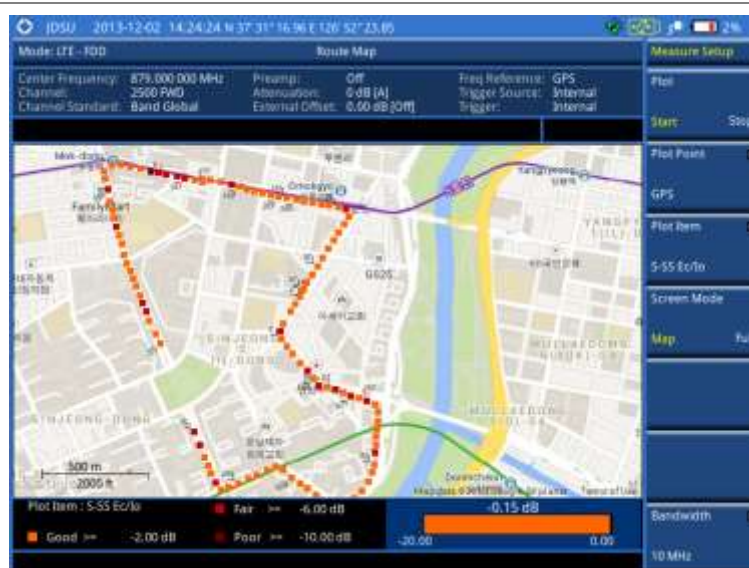
Figure 128 Route map measurement (S-SS Ec/Io) with LTE-FDD OTA signal analyzer
