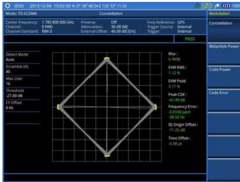
Figure 239 Constellation measurement with TD-SCDMA signal analyzer
