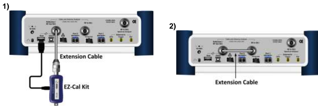
Figure 272 2-port calibration connection with EZ-Cal in vector measurements
