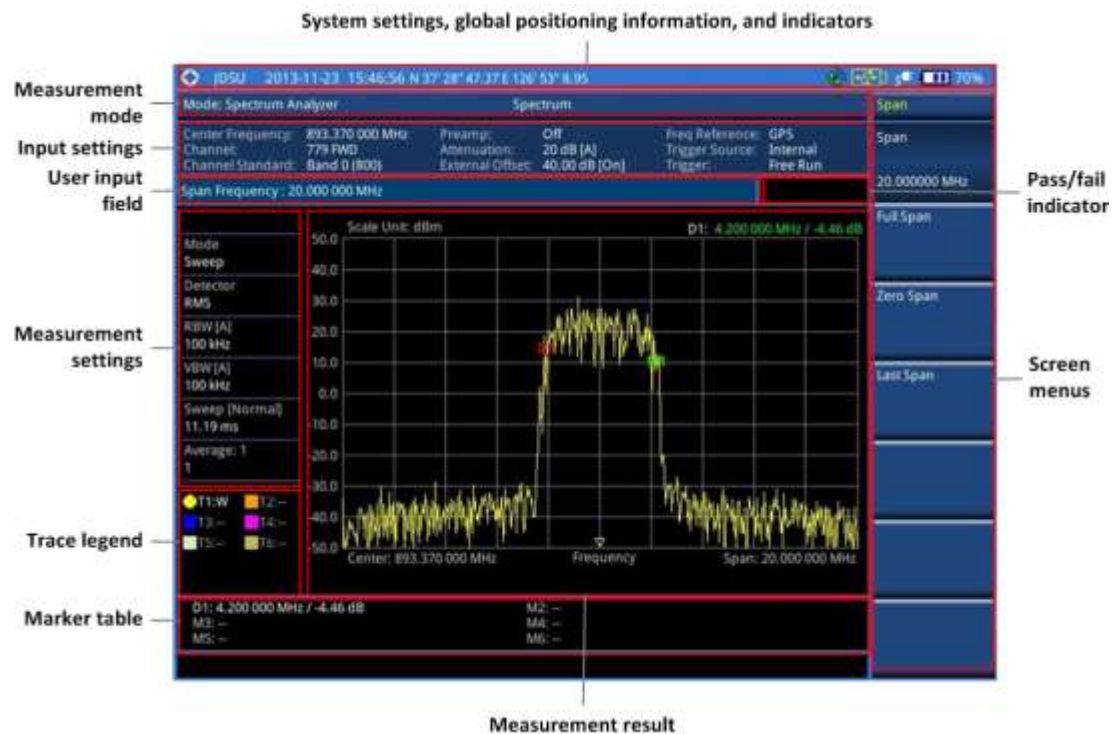
Figure 11 Spectrum measurement screen
