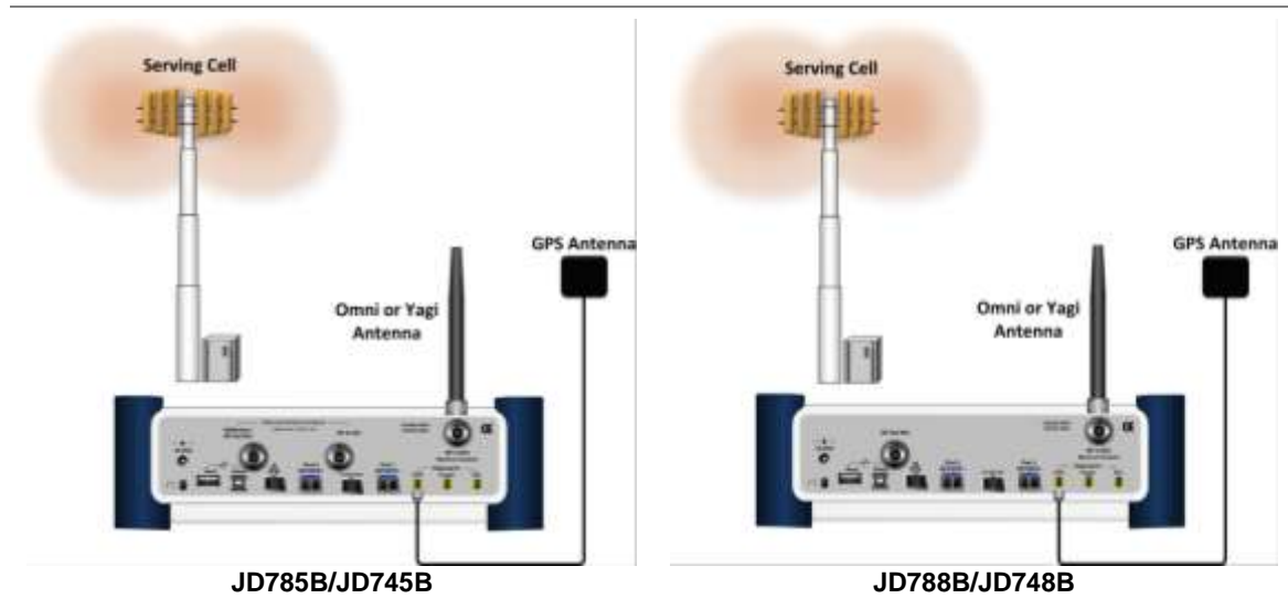
Figure 134 OTA connection
