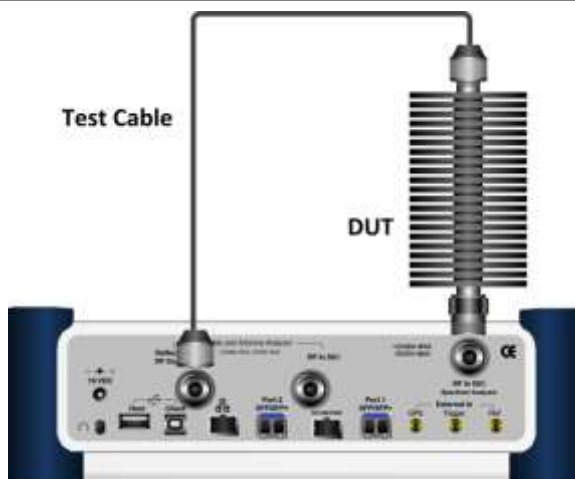
Figure 277 Connection for 2-port scalar measurement
