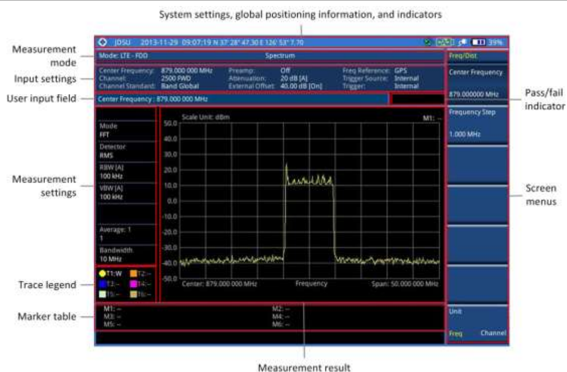
Figure 86 LTE-FDD signal analyzer measurement screen
