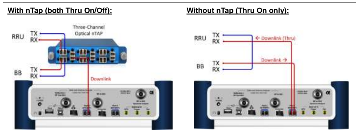
Figure 371 Connection diagram for downlink signal analysis
