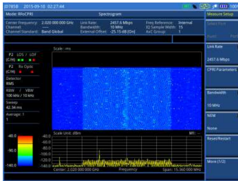
Figure 306 RFoCPRI interference measurement in spectrogram
