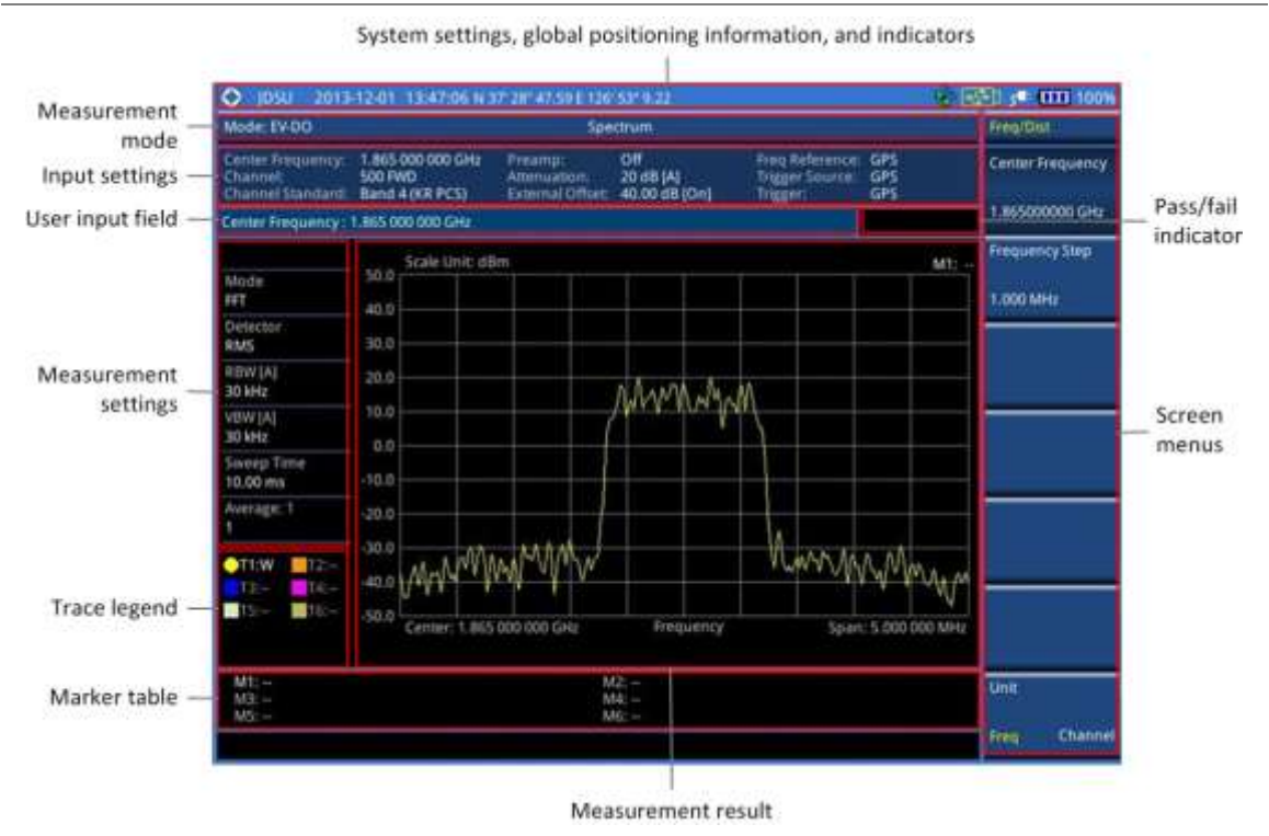
Figure 198 EV-DO signal analyzer measurement screen
