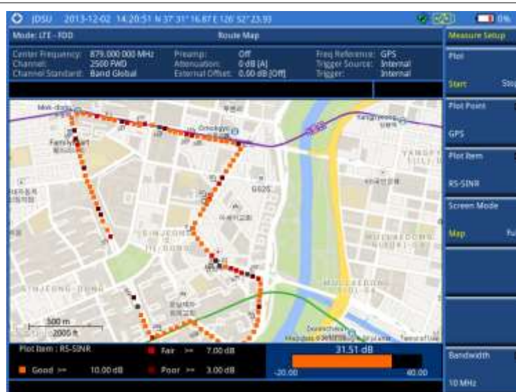
Figure 124 Route map measurement (RS-SINR) with LTE-FDD OTA signal analyzer
