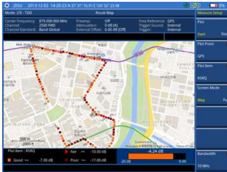
Figure 167 Route map measurement (RSRQ) with LTE-TDD OTA signal analyzer
