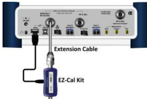
Figure 270 1-port calibration connection with electronic EZ-Cal kit
