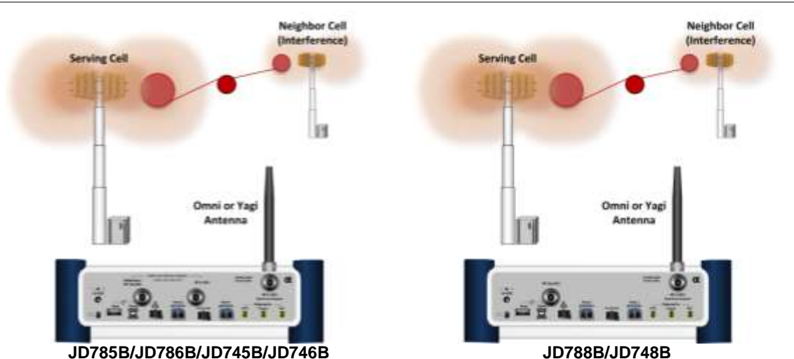
Figure 31 Interference measurement connection
