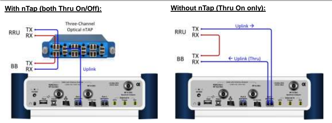
Figure 364 Connection diagram for interference analysis
