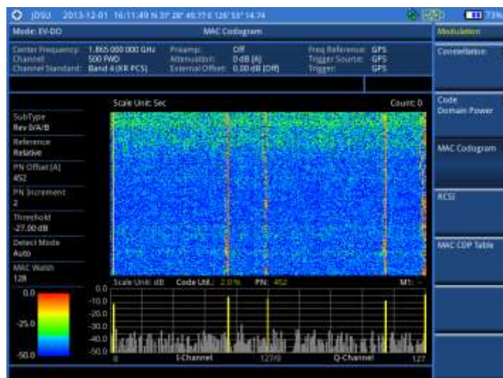
Figure 214 MAC Codogram in full view with EV-DO signal analyzer
