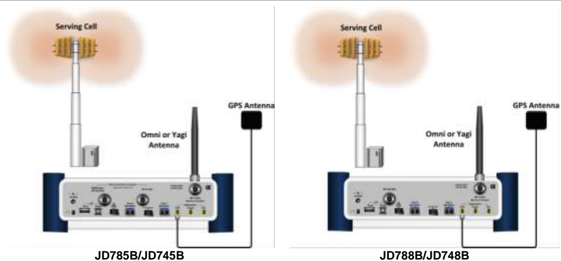
Figure 63 OTA connection
