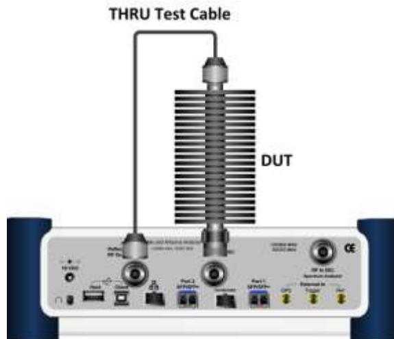
Figure 276 Connection for 2-port vector measurement
