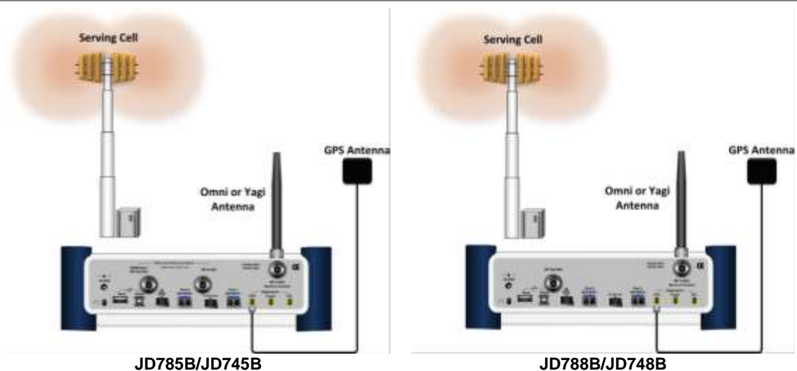
Figure 44 OTA connection
