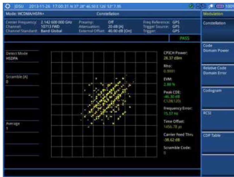
Figure 72 Constellation measurement with WCDMA/HSPA+ signal analyzer
