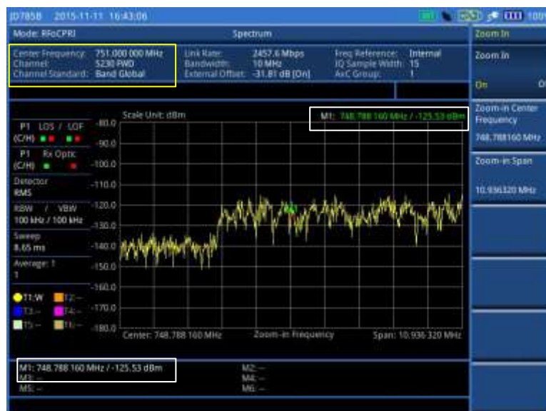
Figure 309 Zoomed-in spectrum view in RFoCPRI interference analyzer
