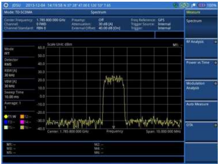
Figure 228 Spectrum measurement screen with TD-SCDMA signal analyzer
