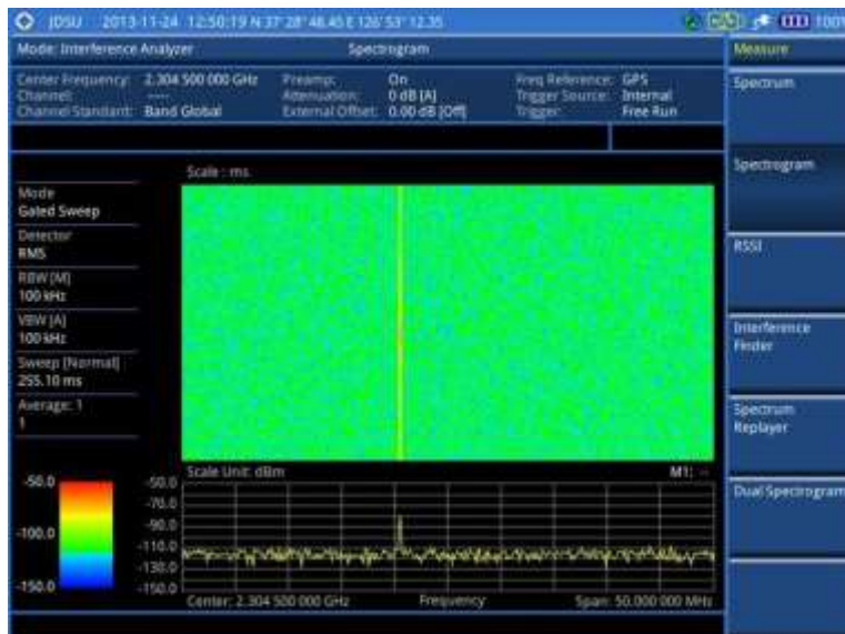
Figure 34 Interference measurement in spectrogram with gated sweep on
