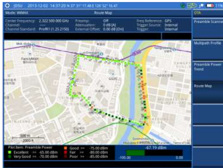
Figure 267 Route map measurement with Mobile WiMAX OTA signal analyzer
