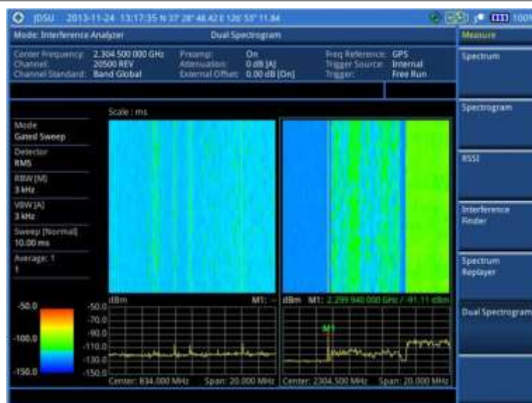
Figure 35 Interference measurement in dual spectrogram view
