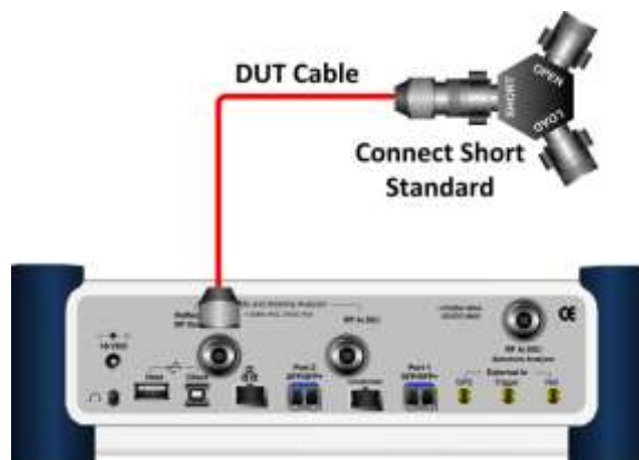
Figure 275 Connection for cable loss (1 port) measurement
