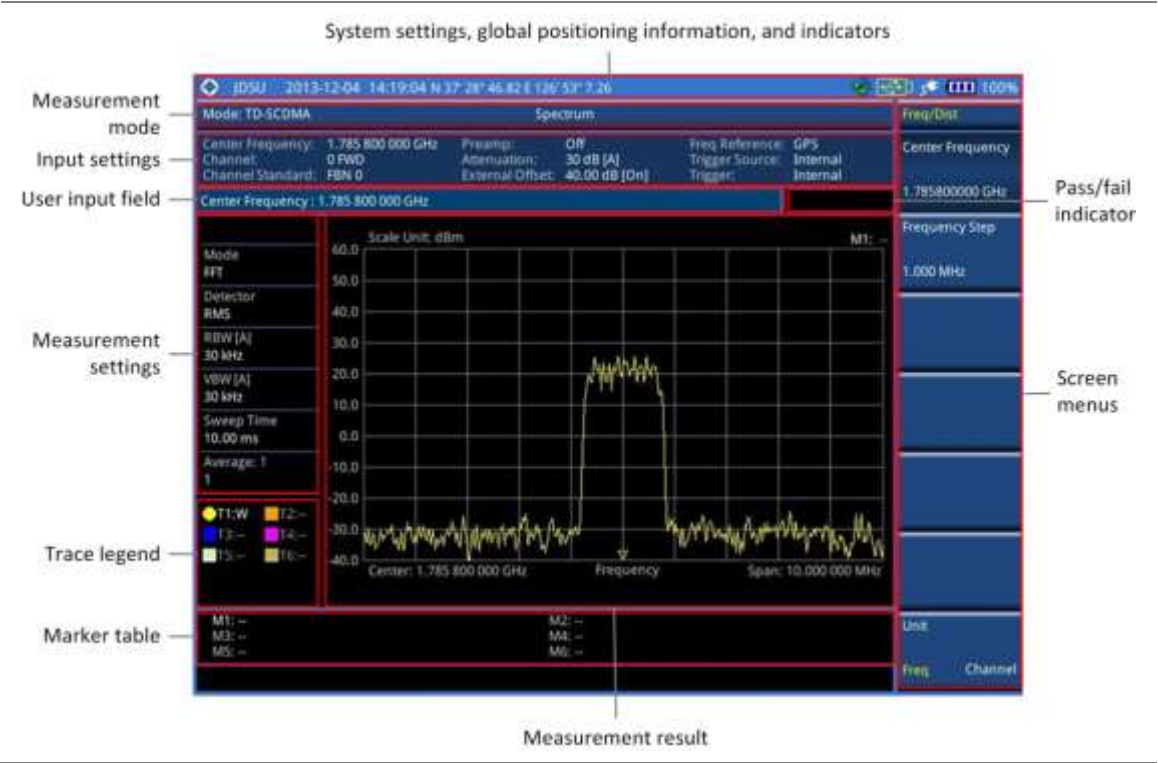
Figure 223 TD-SCDMA signal analyzer measurement screen
