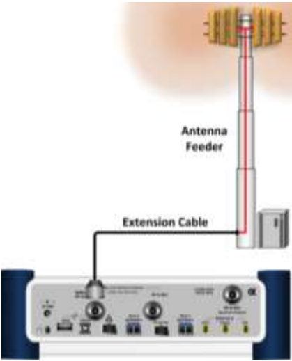
Figure 274 Connection for reflection measurement
