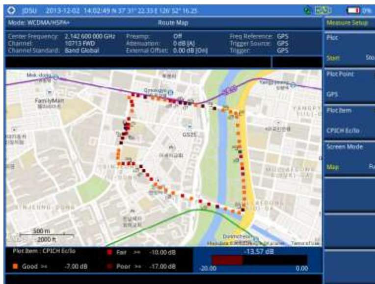
Figure 84 Route map measurement ( CPICH Ec/Io ) with WCDMA/HSPA+ OTA signal analyzer
