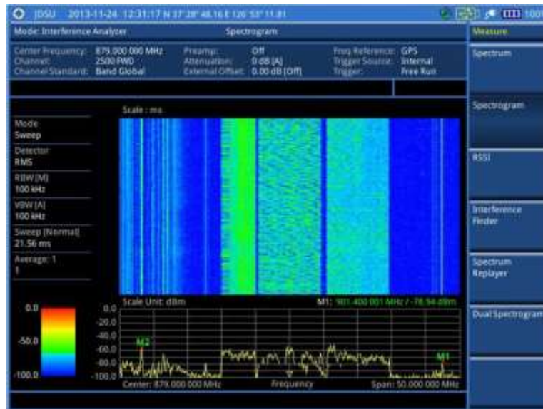
Figure 33 Interference measurement in spectrogram
