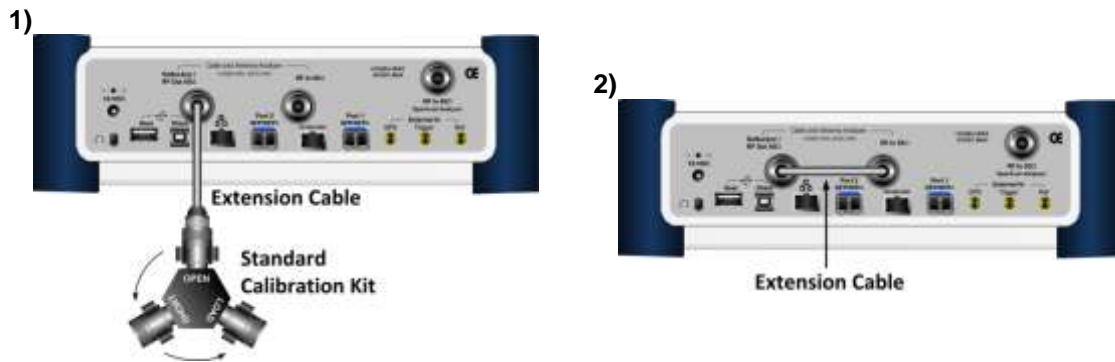
Figure 271 2-port calibration connection with Y-Cal in vector measurements
