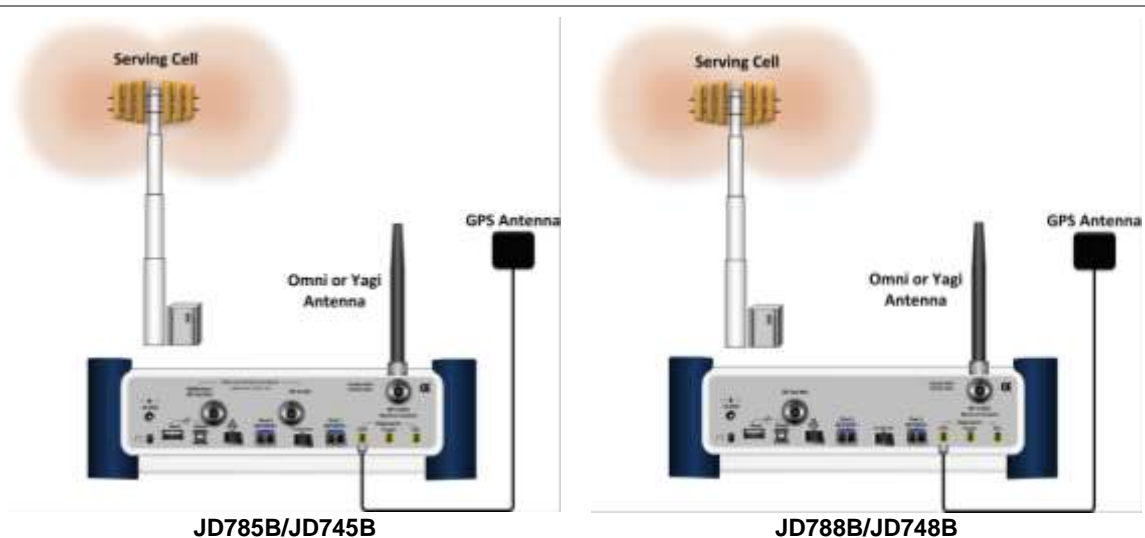
Figure 226 OTA connection
