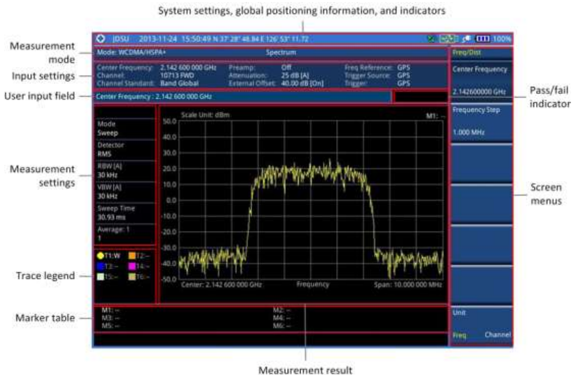
Figure 60 WCDMA/HSPA+ signal analyzer measurement screen
