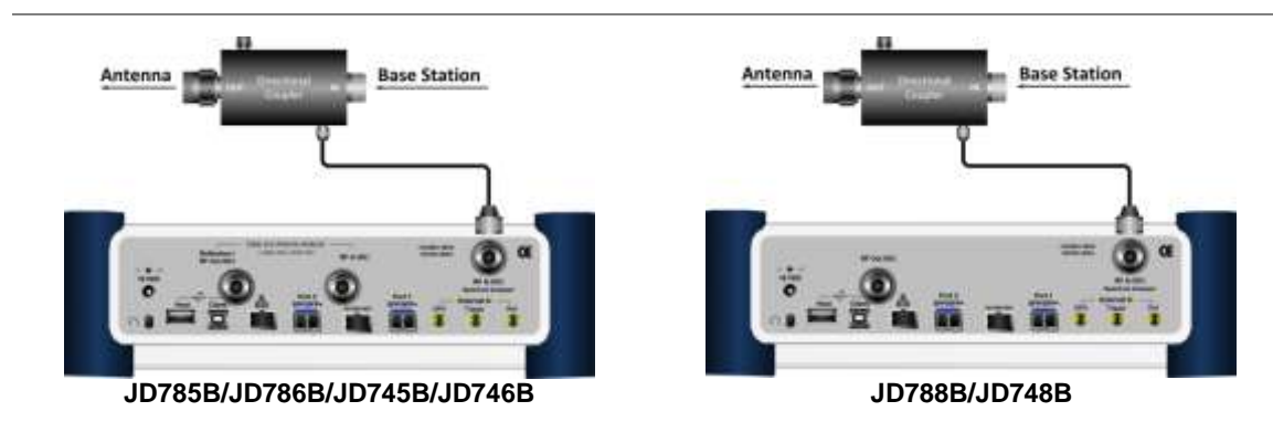
Figure 386 Indirect connection
