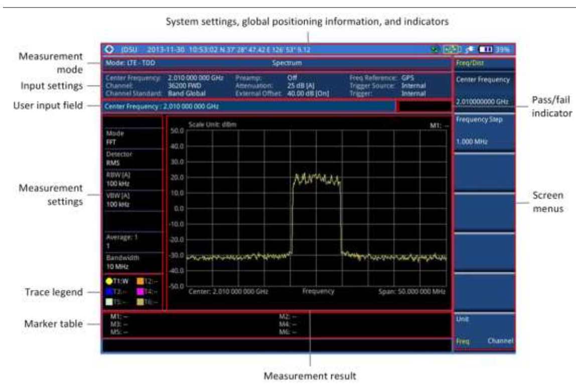
Figure 131 LTE-TDD signal analyzer measurement screen
