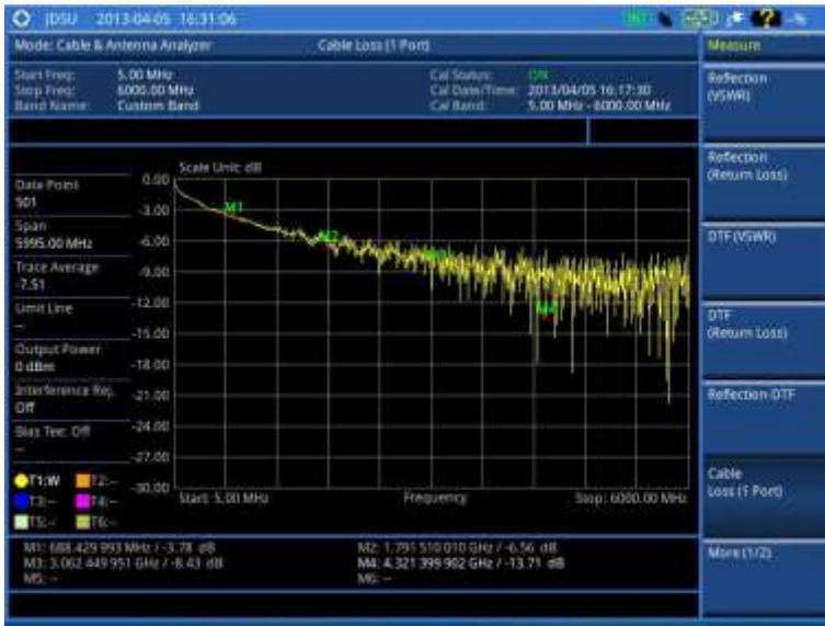
Figure 282 Cable loss (1 port) measurement
