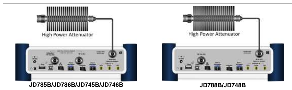
Figure 385 Direct connection
