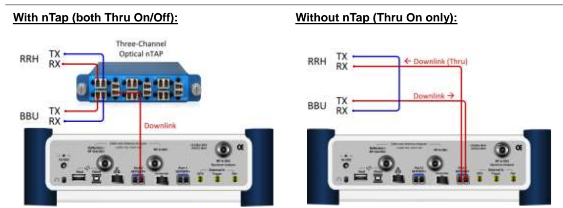
Figure 327 Connection diagram for downlink signal analysis
