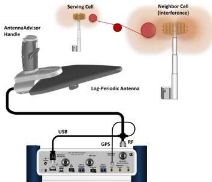
Figure 32 Connection using AntennaAdvisor handle and log-periodic antenna
