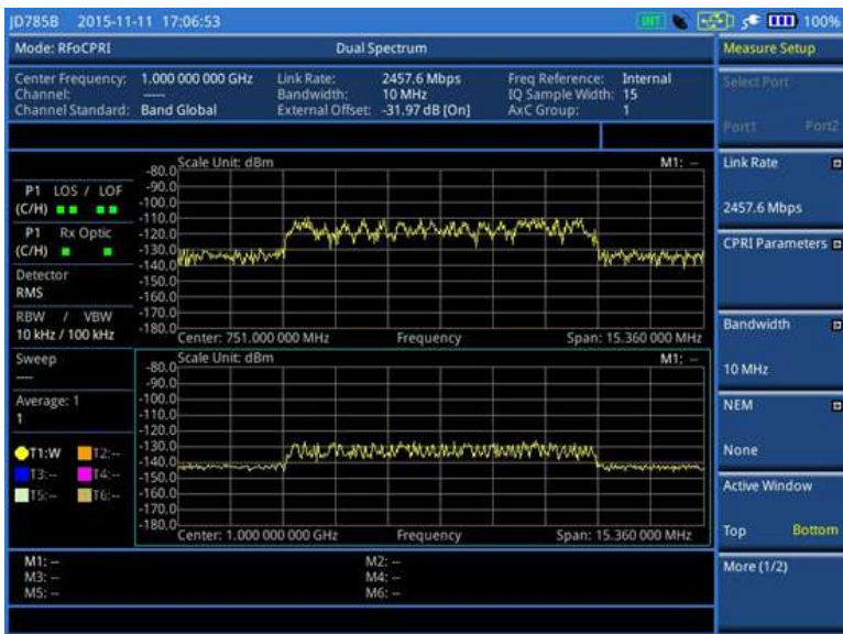
Figure 302 RFoCPRI dual spectrum with dual active trace off
