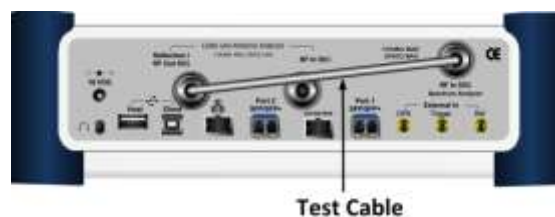
Figure 273 2-port calibration connection in Scalar measurements
