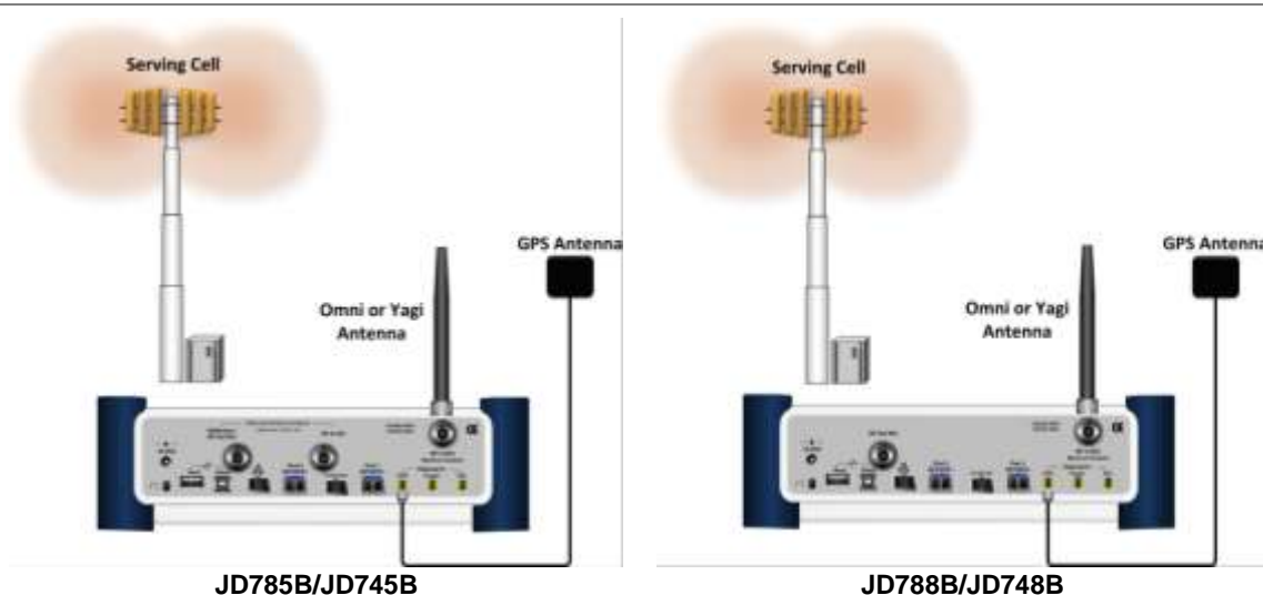
Figure 251 OTA connection
