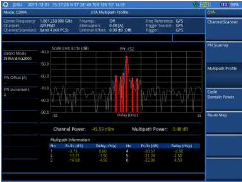
Figure 195 Multipath profile measurement with CDMA OTA signal analyzer
