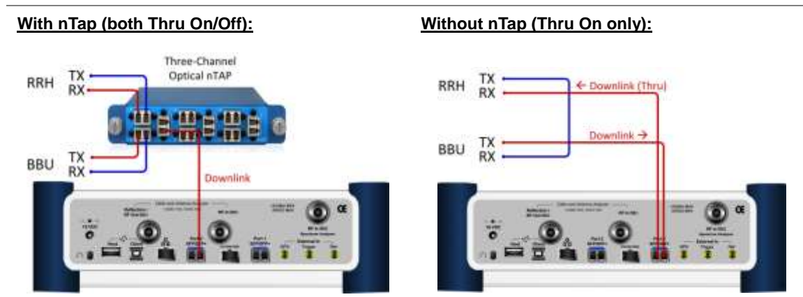
Figure 313 Connection diagram for downlink signal analysis
