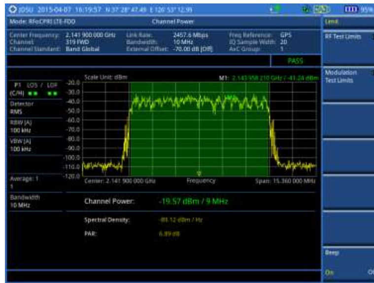
Figure 316 Channel power measurement with RFoCPRI LTE-FDD signal analyzer
