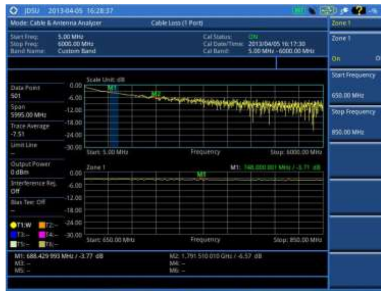
Figure 285 Cable loss (1 port) measurement with zoom
