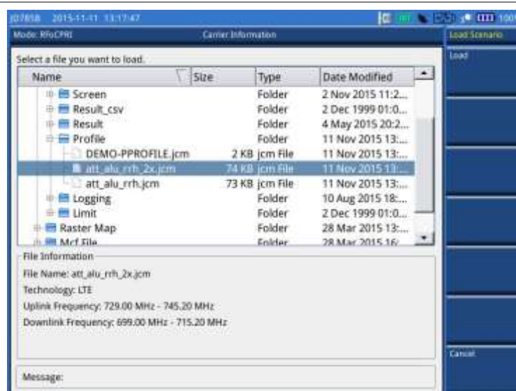
Figure 348 Example of loading a saved RRH profile
