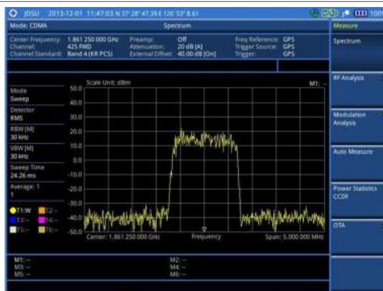
Figure 180 Spectrum measurement screen with CDMA signal analyzer
