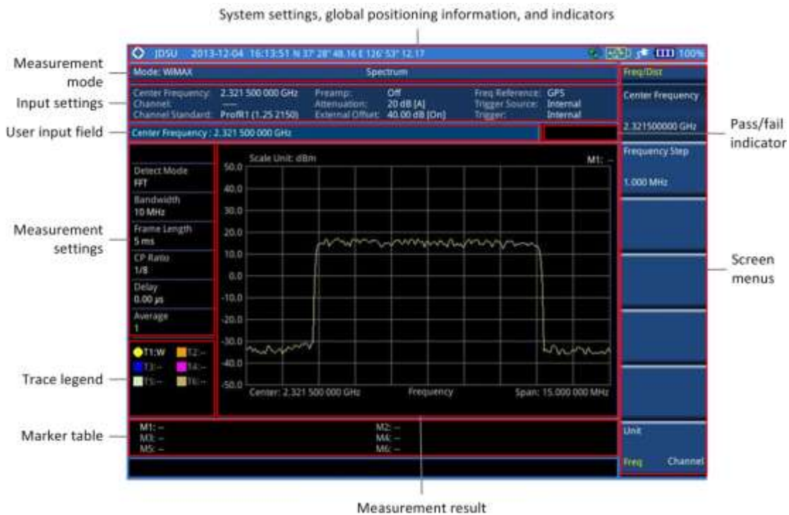
Figure 248 Mobile WiMAX signal analyzer measurement screen
