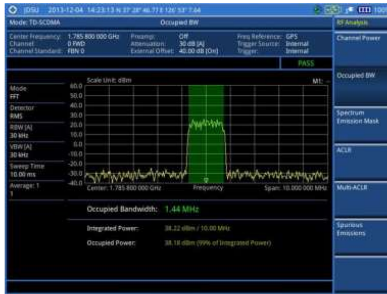
Figure 230 Occupied bandwidth measurement with TD-SCDMA signal analyzer
