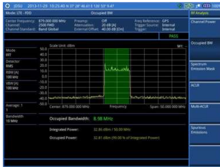
Figure 93 Occupied bandwidth measurement with LTE-FDD signal analyzer
