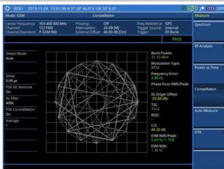
Figure 55 Constellation measurement (PSK on) with GSM signal analyzer
