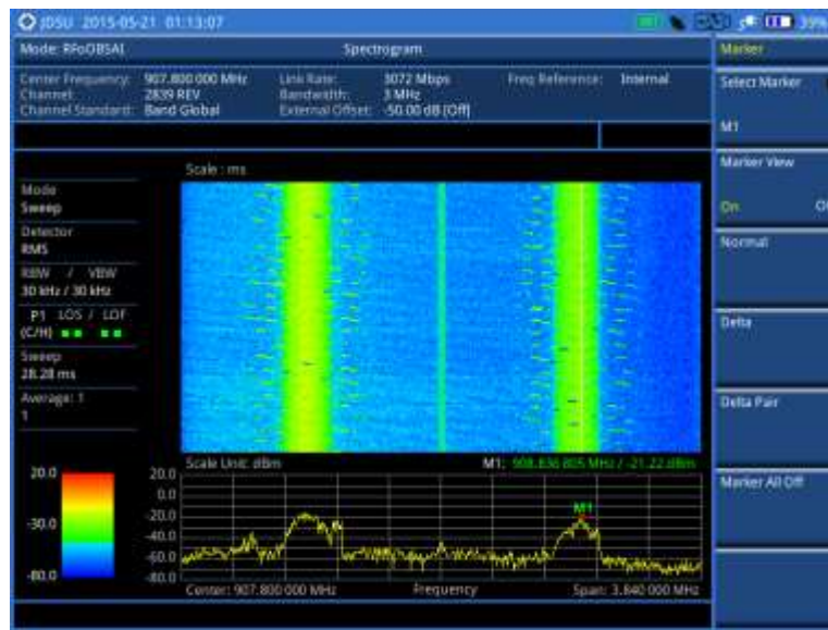
Figure 366 RFoBSAI interference measurement in spectrogram
