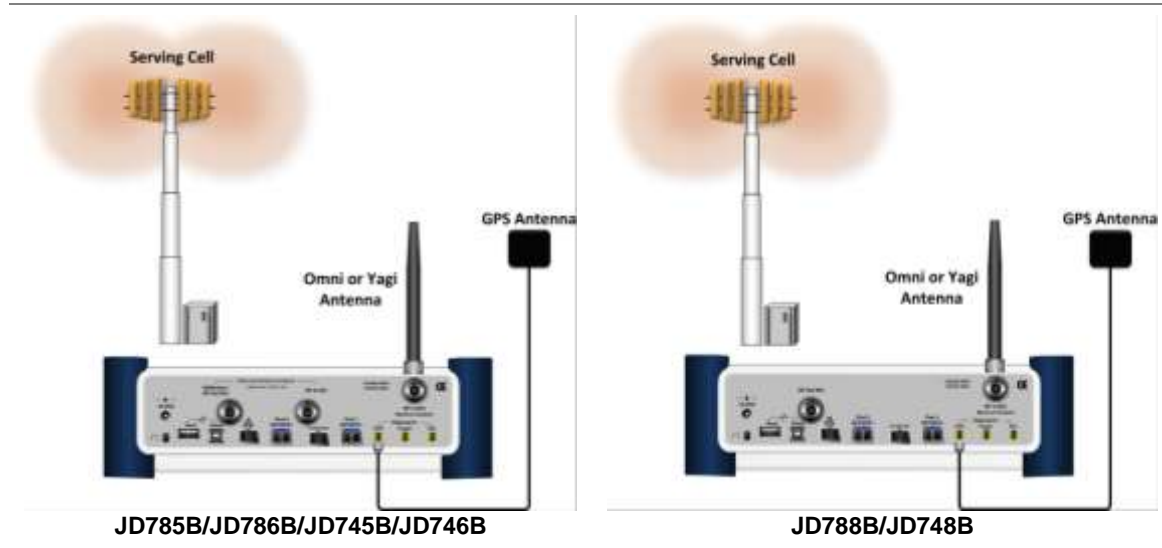
Figure 387 OTA connection
