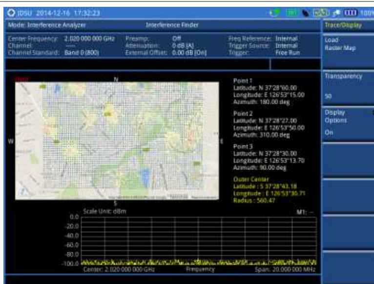
Figure 38 Raster image overlaid on the map in interference finder
