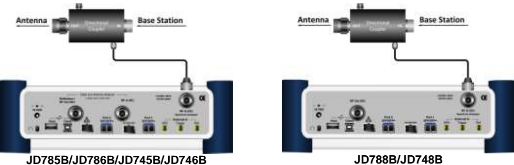
Figure 393 Indirect connection
