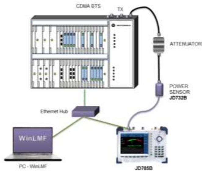
Figure 407 Using external power sensor
