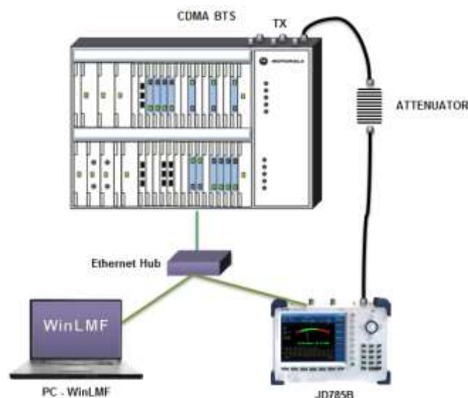
Figure 406 Using internal power sensor
