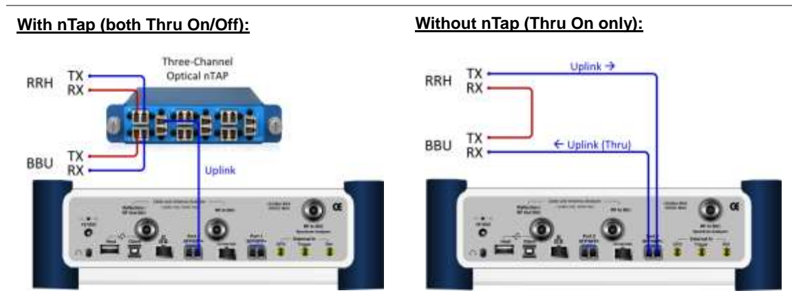
Figure 294 Connection diagram for interference analysis
