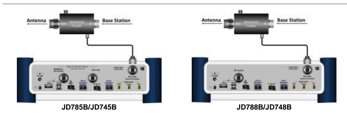
Figure 88 Indirect connection
