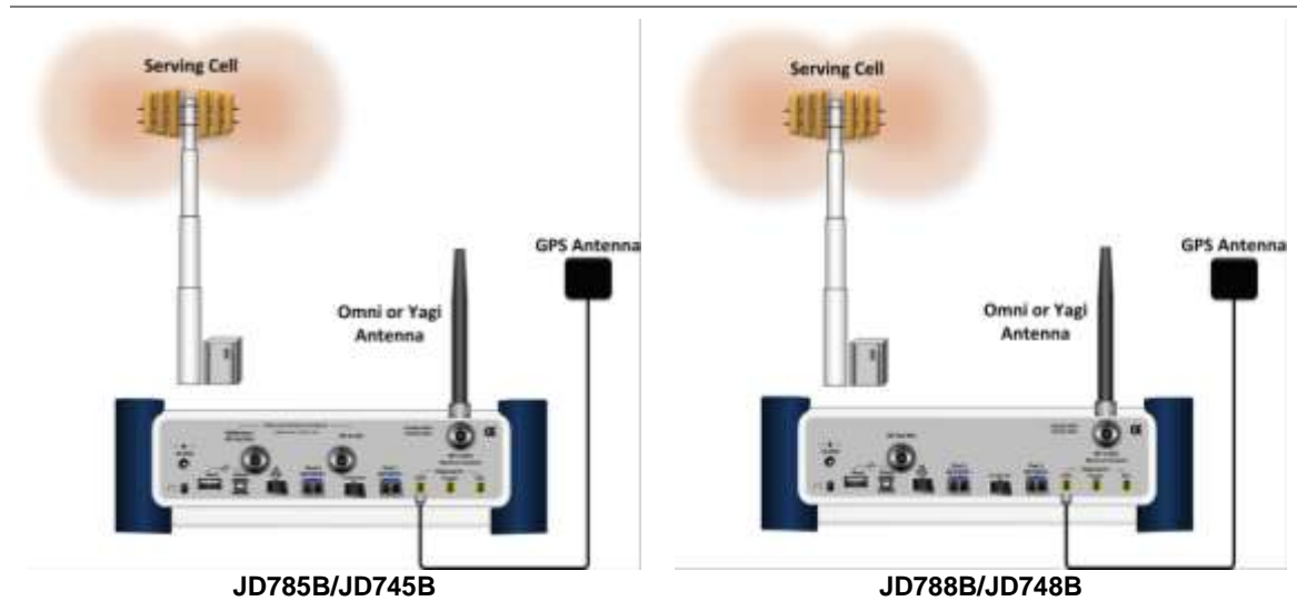
Figure 89 OTA connection
