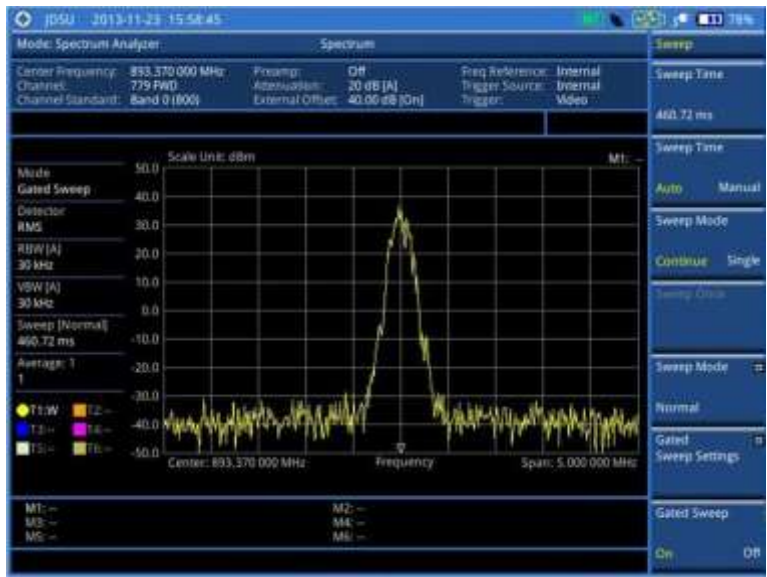
Figure 15 Gate sweep measurement with spectrum analyzer
