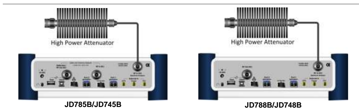
Figure 87 Direct connection
