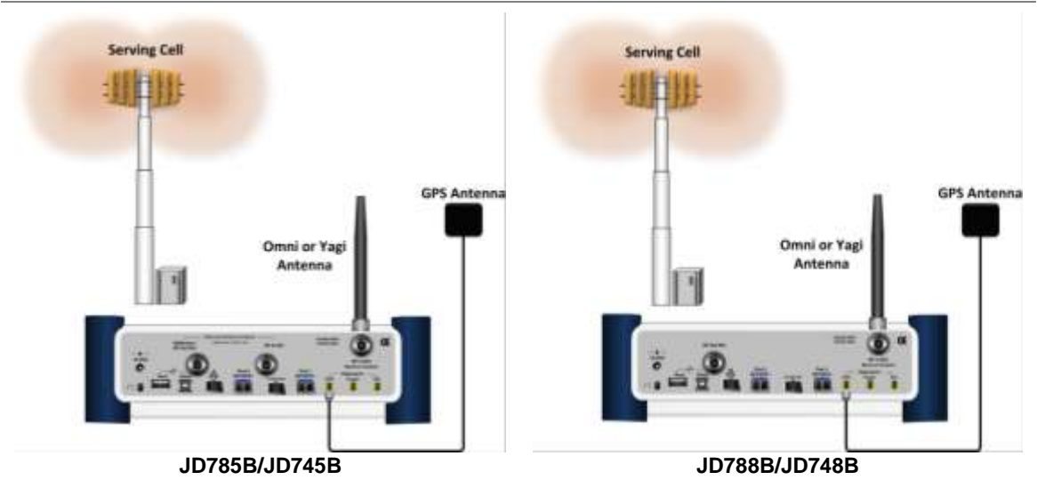
Figure 201 OTA connection
