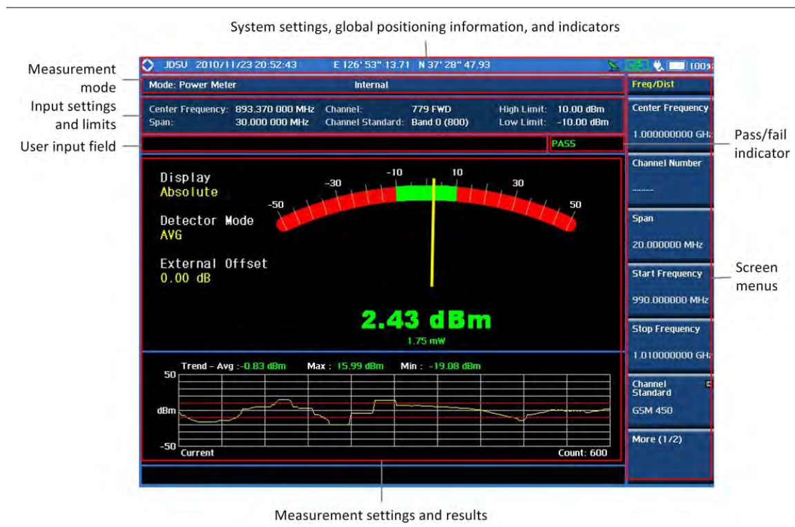
Figure 361 Power measurement screen
