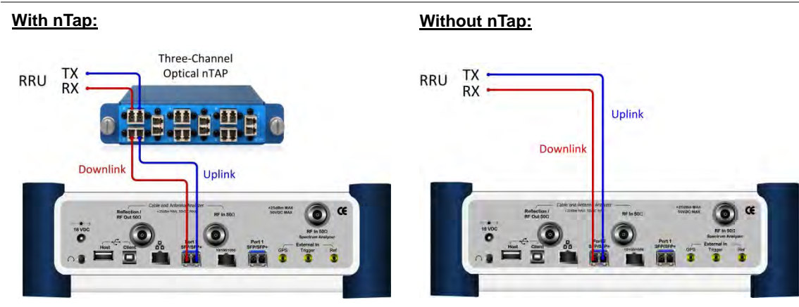
Figure 332 Connection diagram for Layer-2 term testing mode
