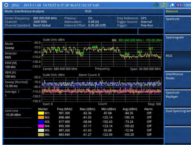
Figure 32 Interference measurement in RSSI
