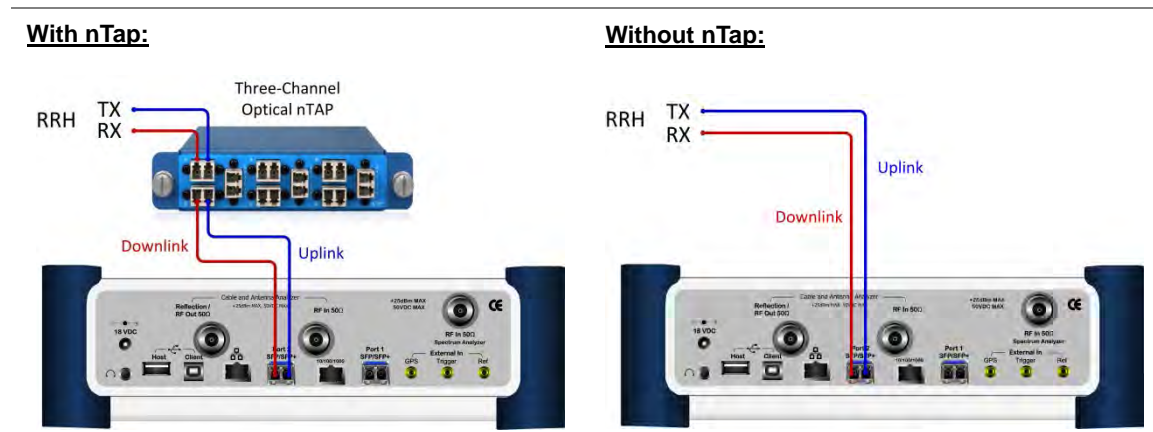
Figure 288 Connection diagram for Layer-2 term testing mode
