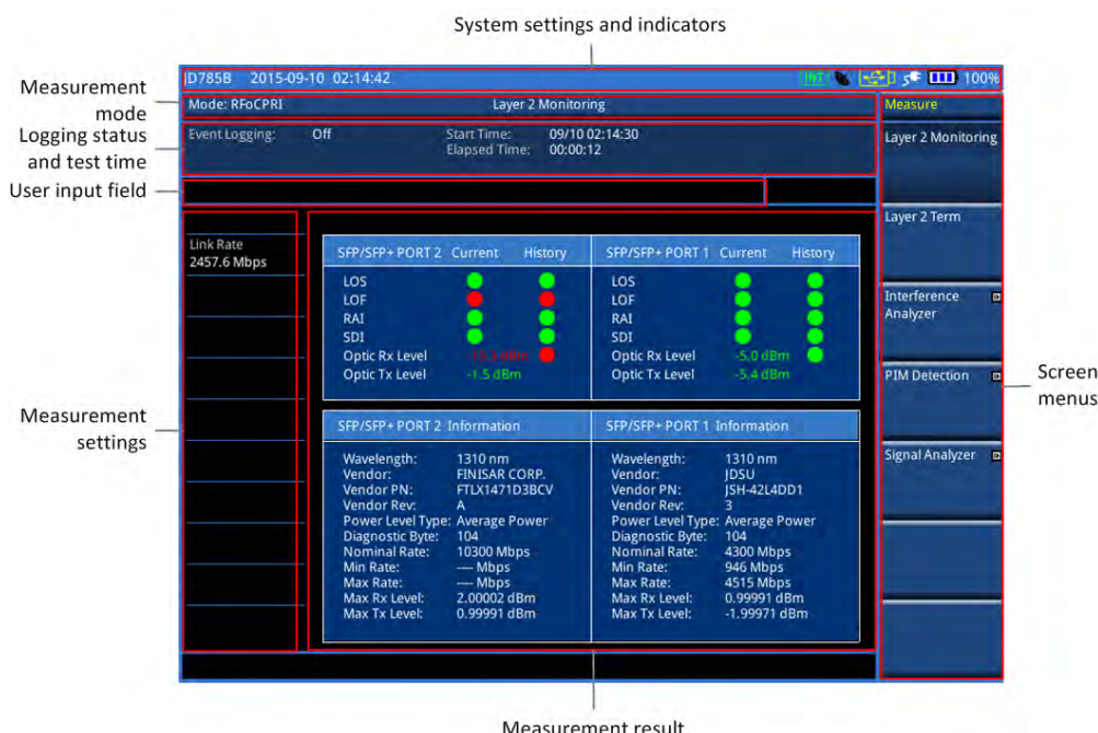
Figure 285 RFoCPRI analysis screen
