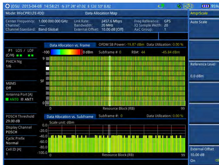
Figure 315 Data allocation map measurement with RFoCPRI LTE-FDD signal analyzer
