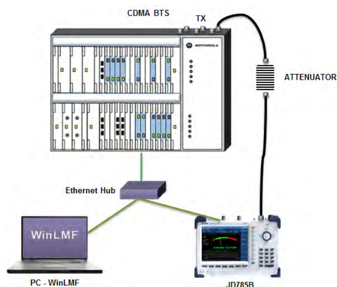
Figure 373 Using internal power sensor
