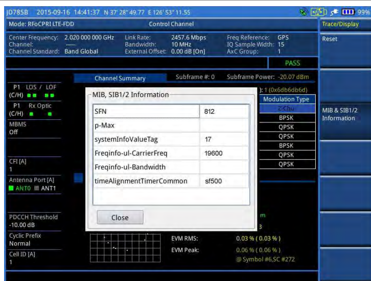
Figure 304 Decoded MIB & SIB1/2 information in RFoCPRI LTE-FDD signal analyzer
