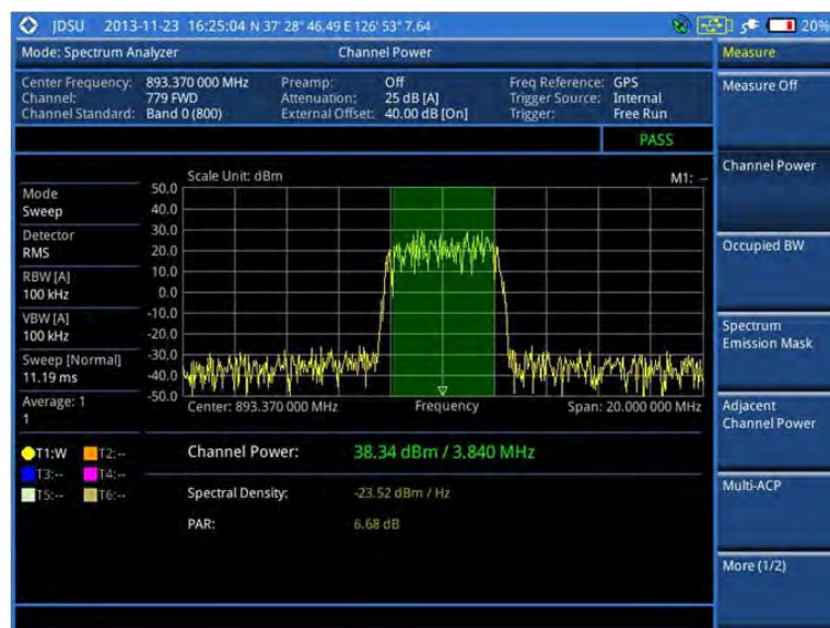
Figure 13 Channel power measurement with spectrum analyzer
