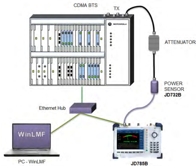
Figure 374 Using external power sensor
