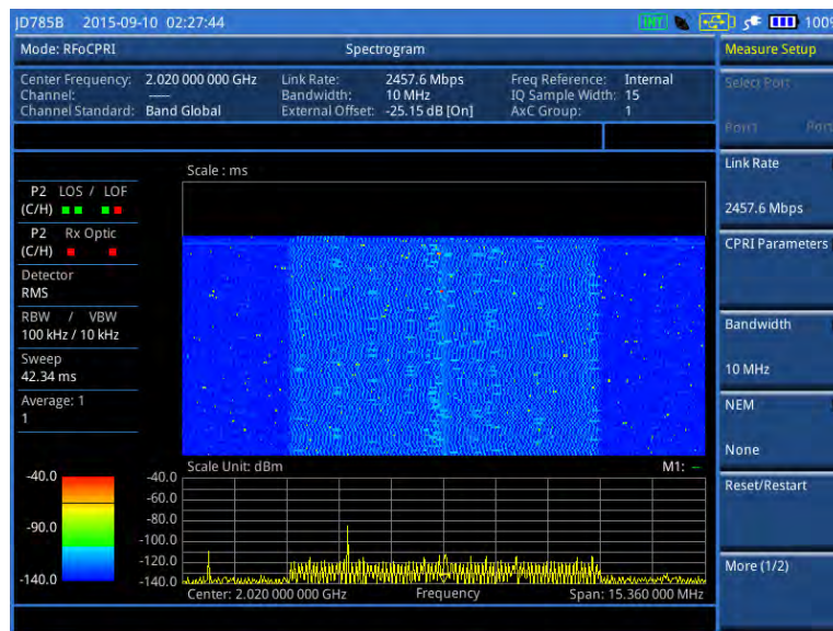
Figure 297 RFoCPRI interference measurement in spectrogram
