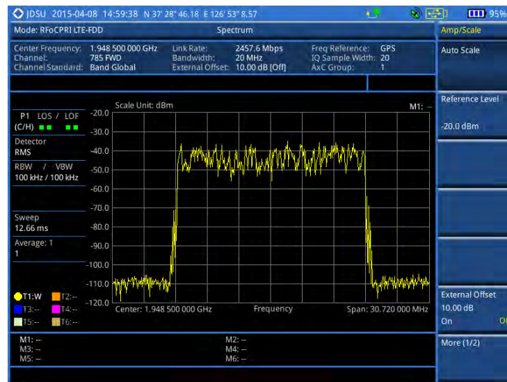
Figure 305 Spectrum measurement with RFoCPRI LTE-FDD signal analyzer
