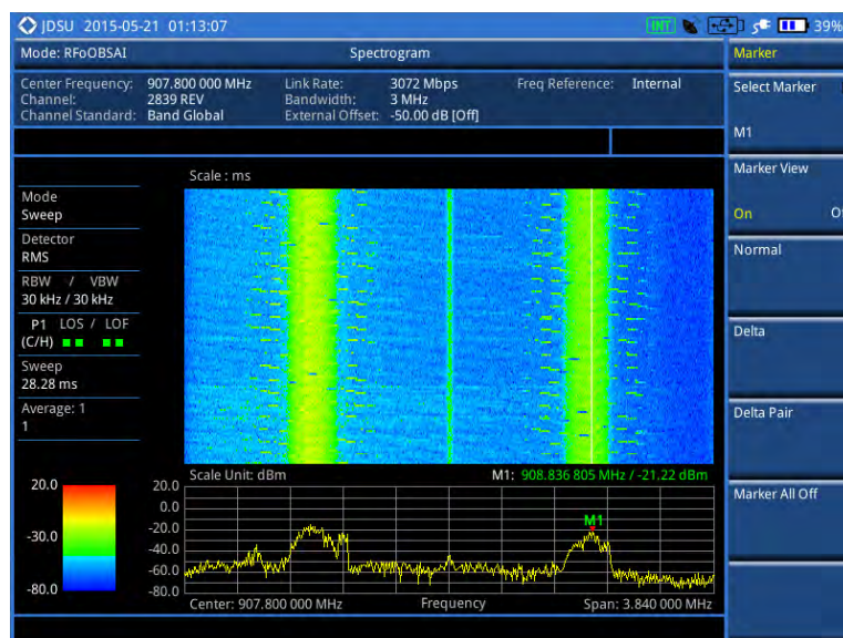
Figure 336 RFoOBSAI interference measurement in spectrogram
