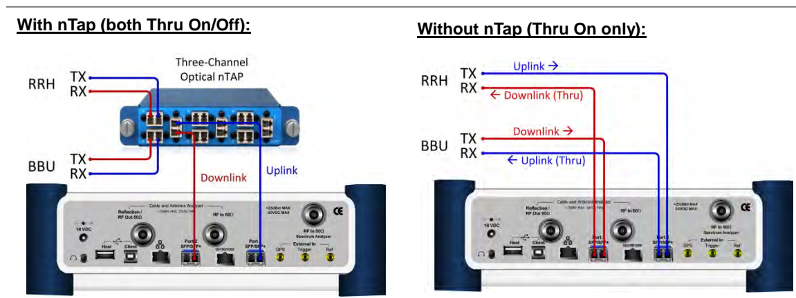
Figure 286 Connection diagram for Layer-2 monitoring mode
