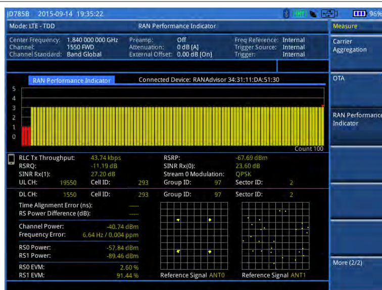
Figure 170 RAN performance indicator with LTE-TDD signal analyzer
