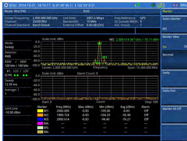
Figure 299 RFoCPRI interference measurement in RSSI
