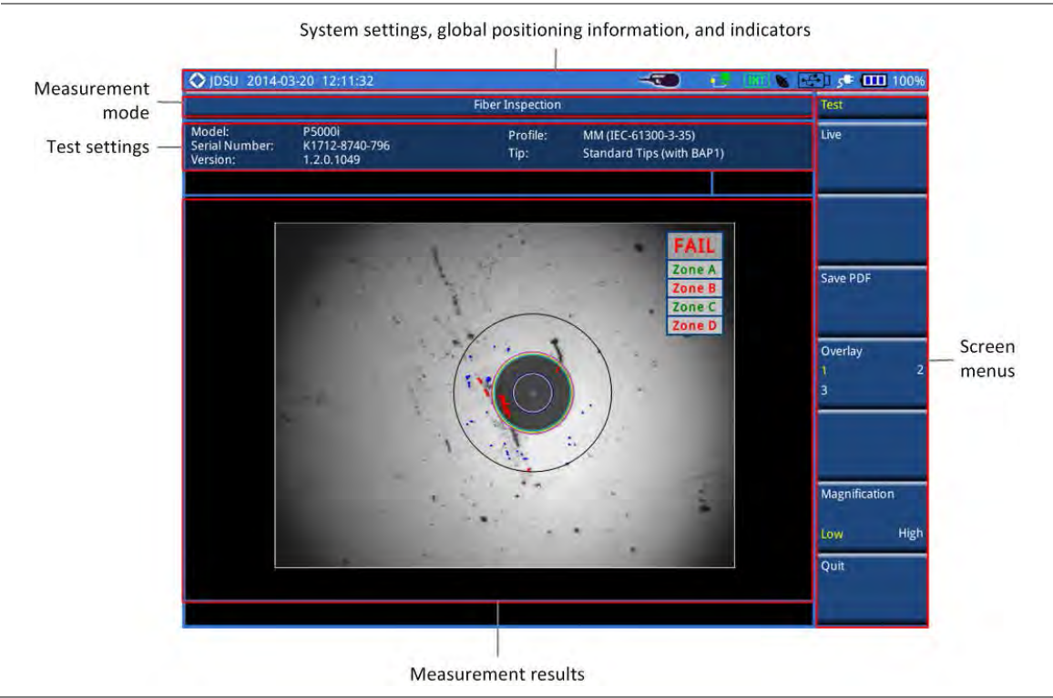
Figure 369 Fiber inspection screen
