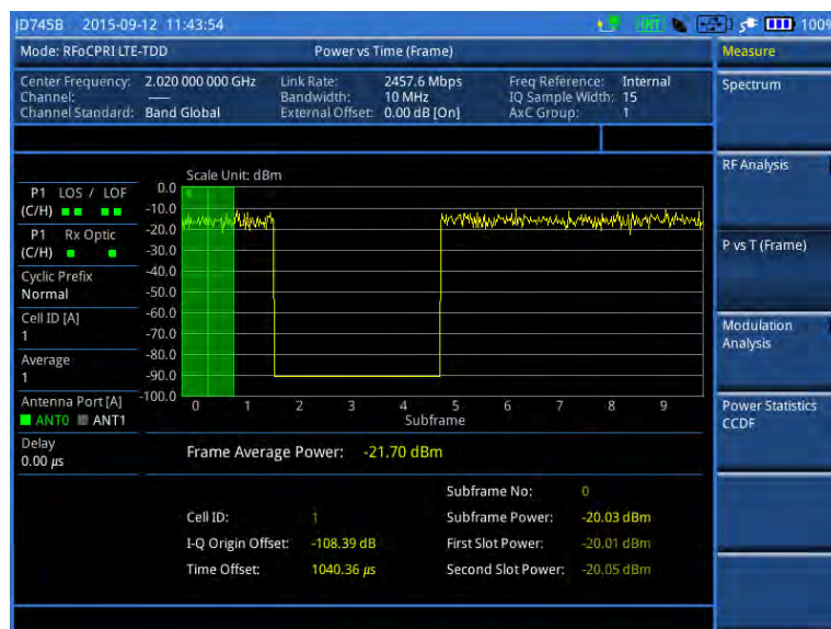
Figure 321 Power vs. time (frame) measurement with RFoCPRI LTE-TDD signal analyzer
