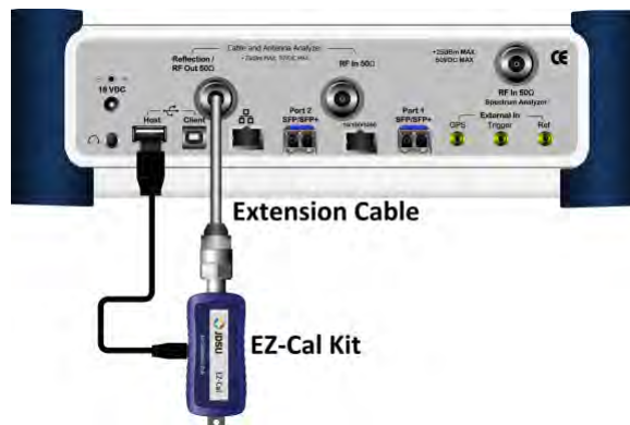
Figure 266 1-port calibration connection with electronic EZ-Cal kit
