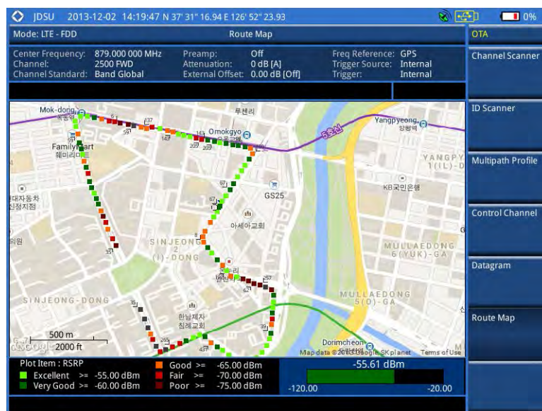
Figure 118 Route map measurement (RSRP) with LTE-FDD OTA signal analyzer
