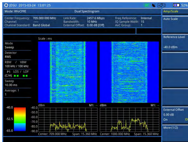
Figure 298 RFoCPRI dual spectrogram analysis
