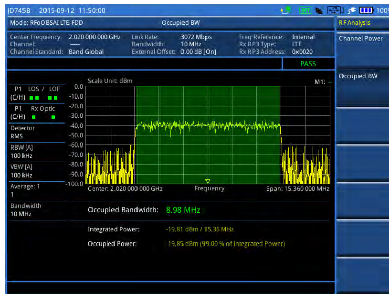
Figure 344 Occupied bandwidth measurement with RFoBSAI LTE-FDD signal analyzer
