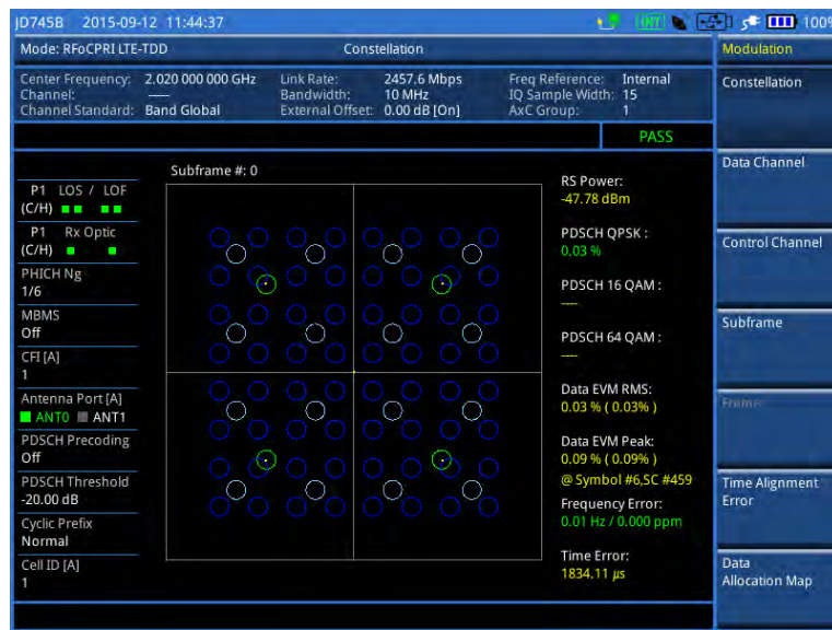
Figure 322 Constellation measurement with RFoCPRI LTE-TDD signal analyzer
