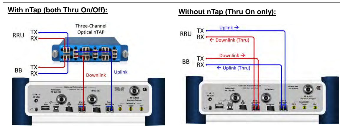
Figure 330 Connection diagram for Layer-2 monitoring mode
