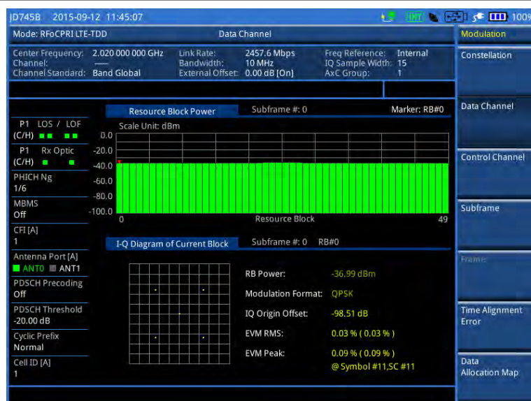
Figure 323 Data channel measurement with RFoCPRI LTE-FDD signal analyzer
