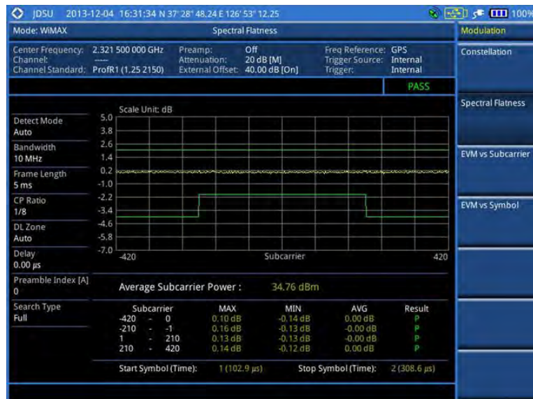
Figure 256 Spectral flatness measurement with Mobile WiMAX signal analyzer
