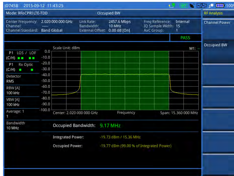
Figure 320 Occupied bandwidth measurement with RFoCPRI LTE-TDD signal analyzer
