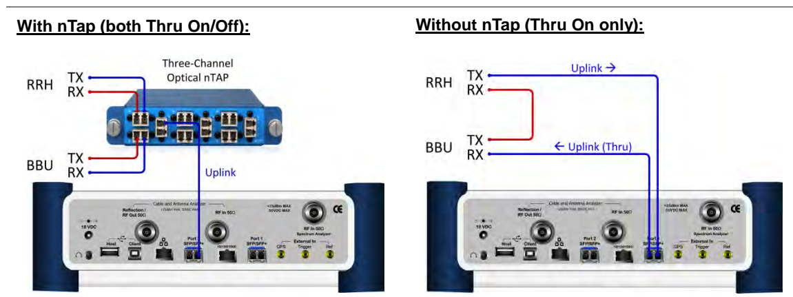
Figure 301 Connection diagram for PIM detection
