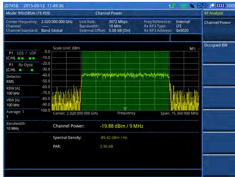
Figure 343 Channel power measurement with RFoBSAI LTE-FDD signal analyzer
