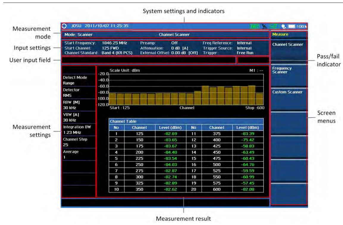
Figure 354 Channel scanner screen
