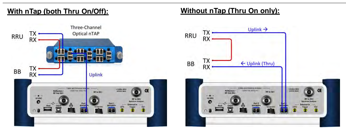
Figure 339 Connection diagram for PIM detection
