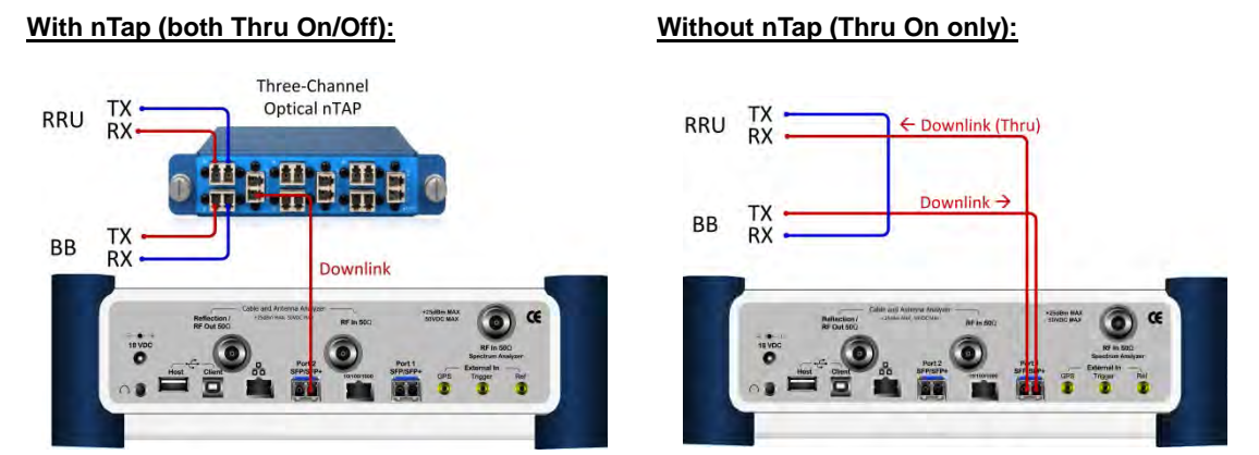
Figure 341 Connection diagram for downlink signal analysis
