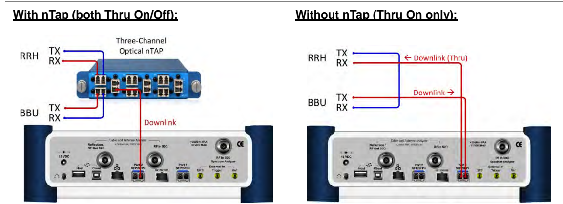
Figure 317 Connection diagram for downlink signal analysis
