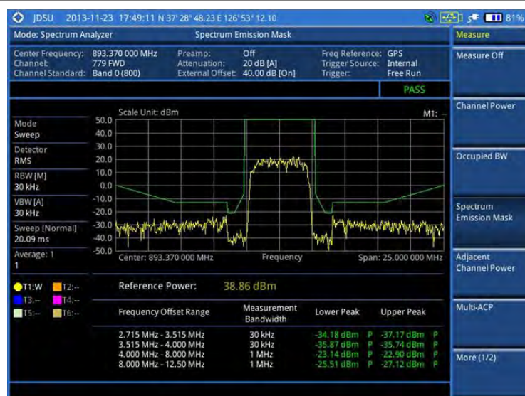
Figure 15 Spectrum emission mask measurement with spectrum analyzer
