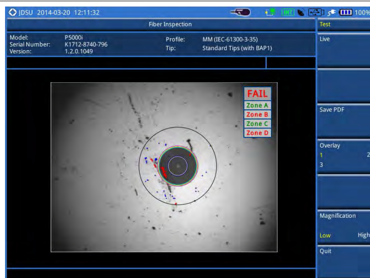
Figure 371 Analyzed fiber image and fiber inspection result
