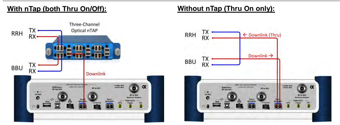
Figure 303 Connection diagram for downlink signal analysis
