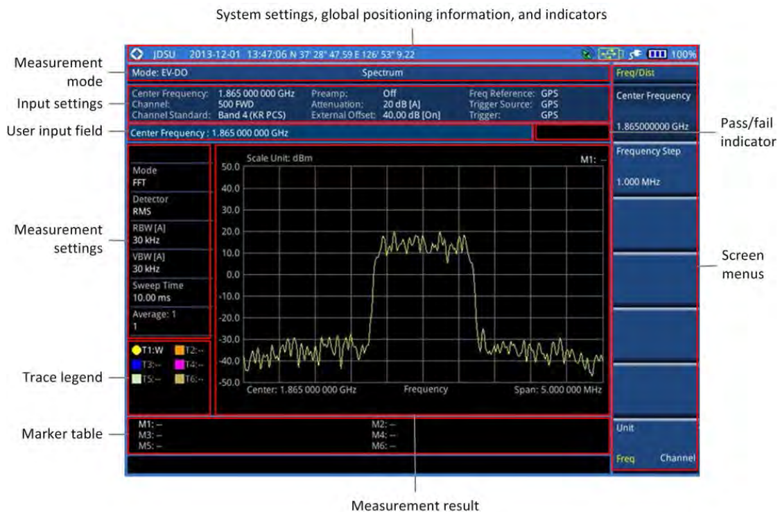
Figure 194 EV-DO signal analyzer measurement screen
