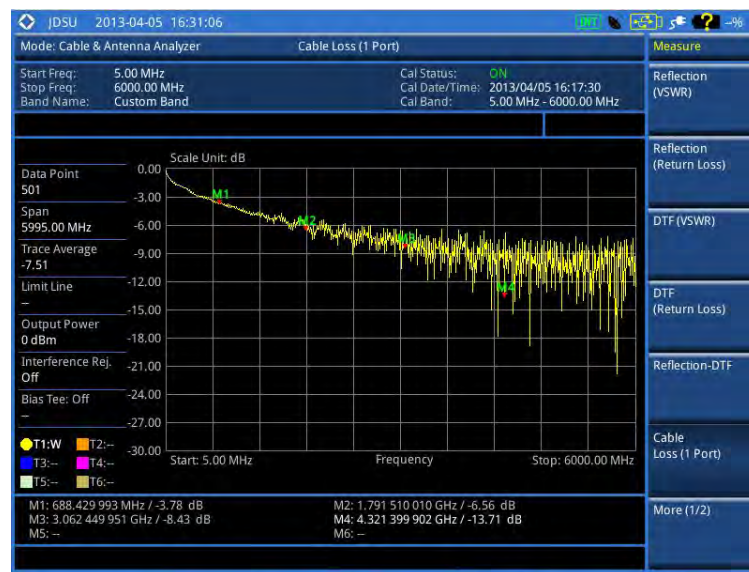
Figure 280 Cable loss (1 port) measurement
