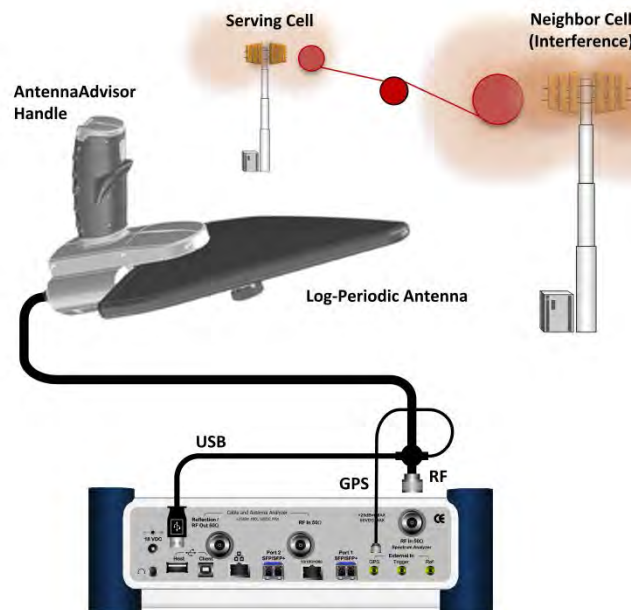
Figure 28 Connection using AntennaAdvisor handle and log-periodic antenna
