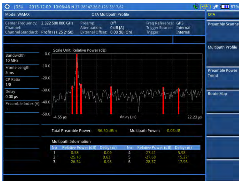
Figure 261 Multipath profile measurement with Mobile WiMAX OTA signal analyzer
