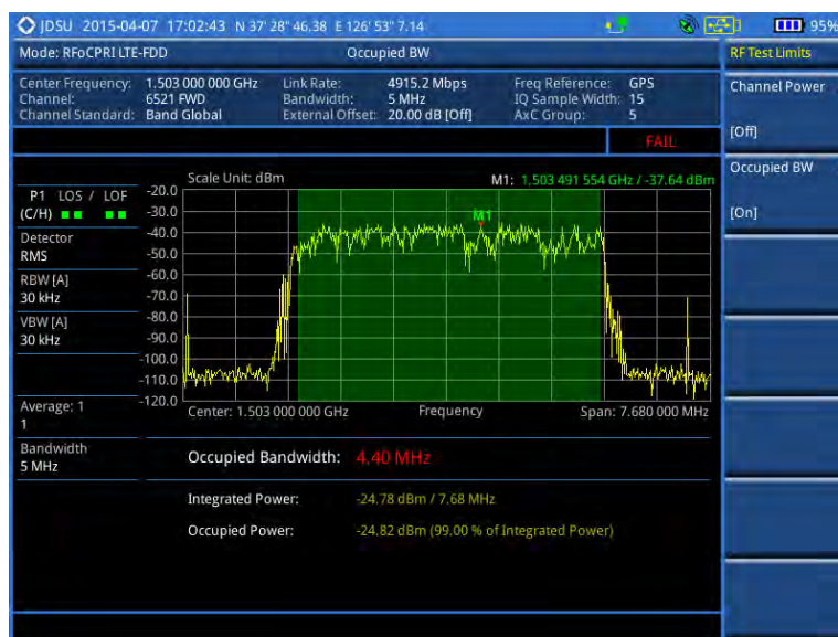
Figure 307 Occupied bandwidth measurement with RFoCPRI LTE-FDD signal analyzer
