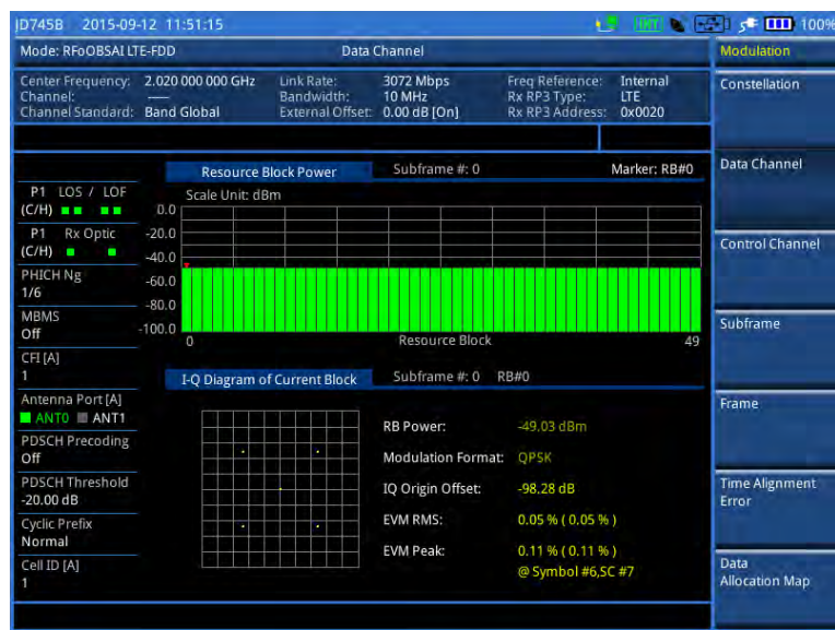
Figure 347 Data channel measurement with RFoOBSAI LTE-FDD signal analyzer
