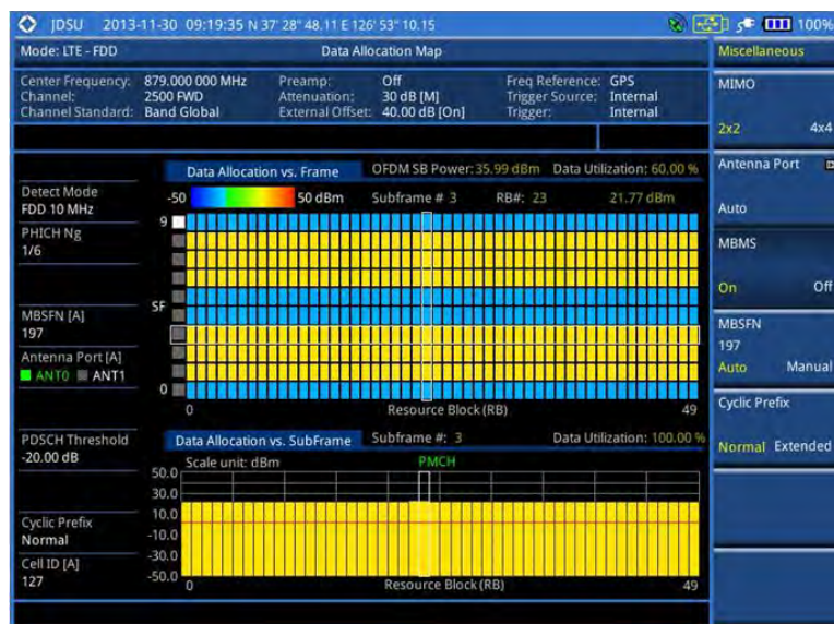
Figure 108 Data allocation map measurement with LTE-FDD signal analyzer (MBMS On)
