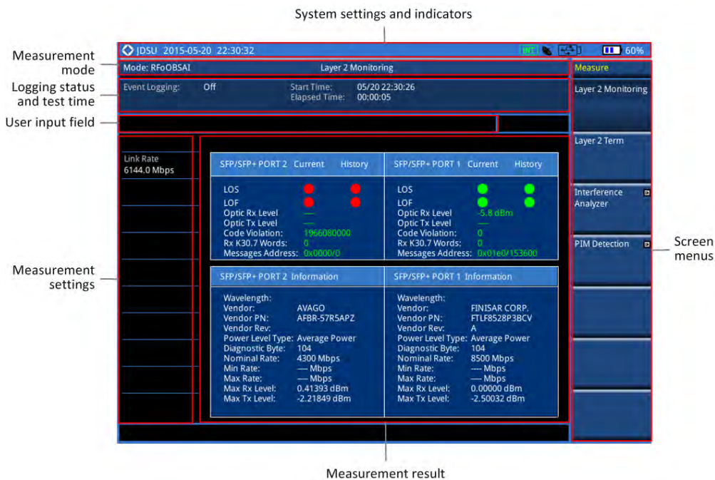
Figure 329 RFoBSAI analysis screen
