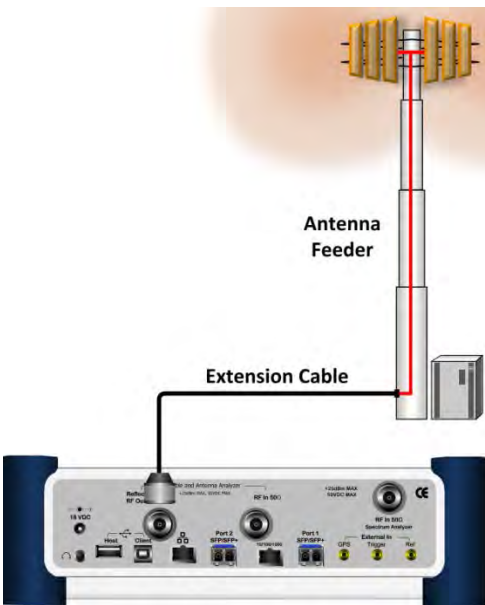
Figure 270 Connection for reflection measurement
