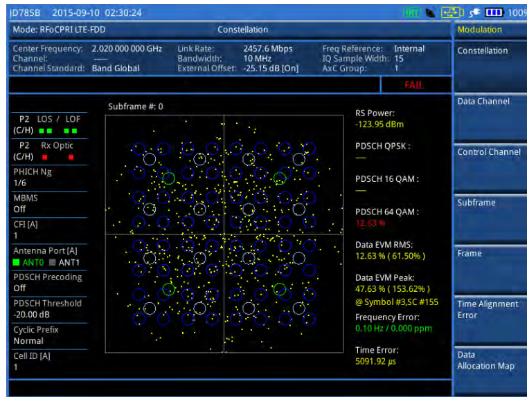
Figure 309 Constellation measurement with RFoCPRI LTE-FDD signal analyzer
