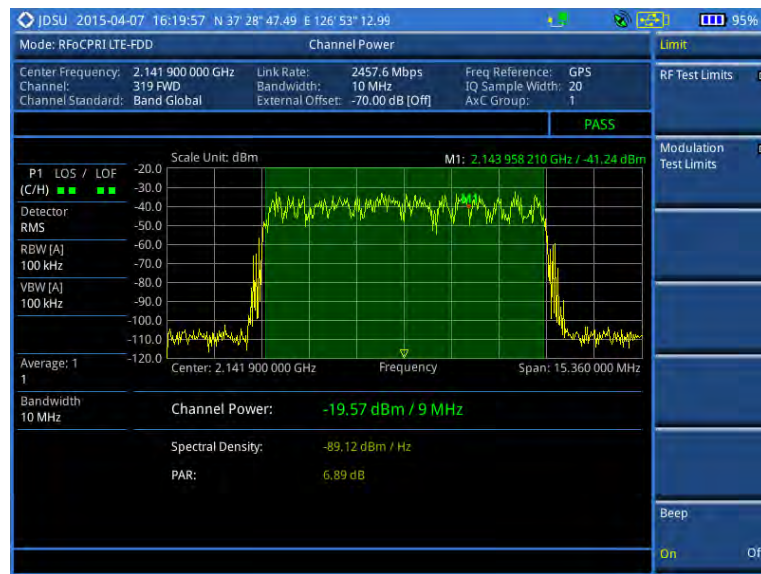
Figure 306 Channel power measurement with RFoCPRI LTE-FDD signal analyzer
