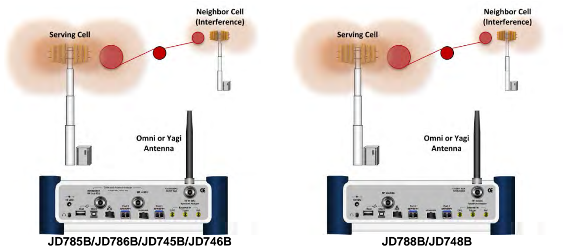
Figure 27 Interference measurement connection
