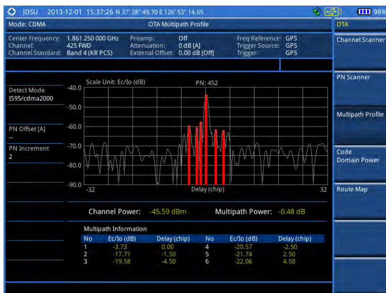
Figure 191 Multipath profile measurement with CDMA OTA signal analyzer
