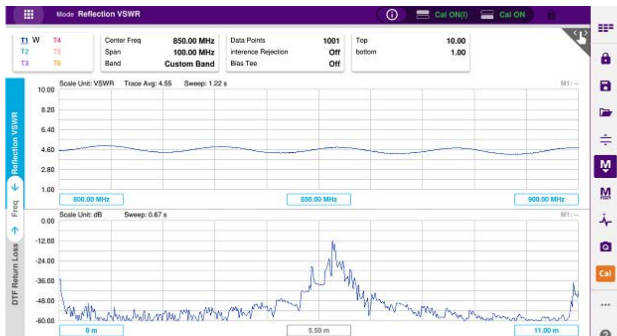
DTF VSWR & Smith chart measurement screen (vertical layout)
